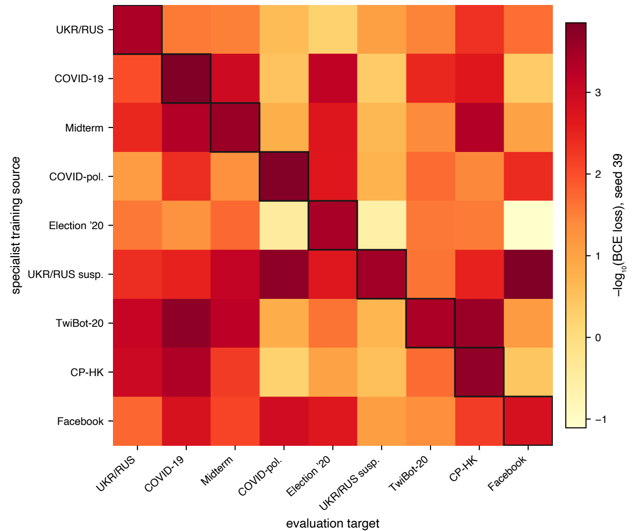
SAMGPT · GraphCL
