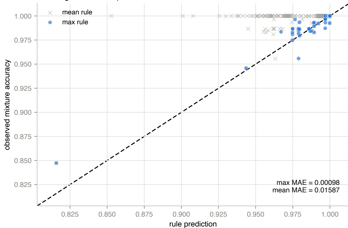
243 target-level comparisons
