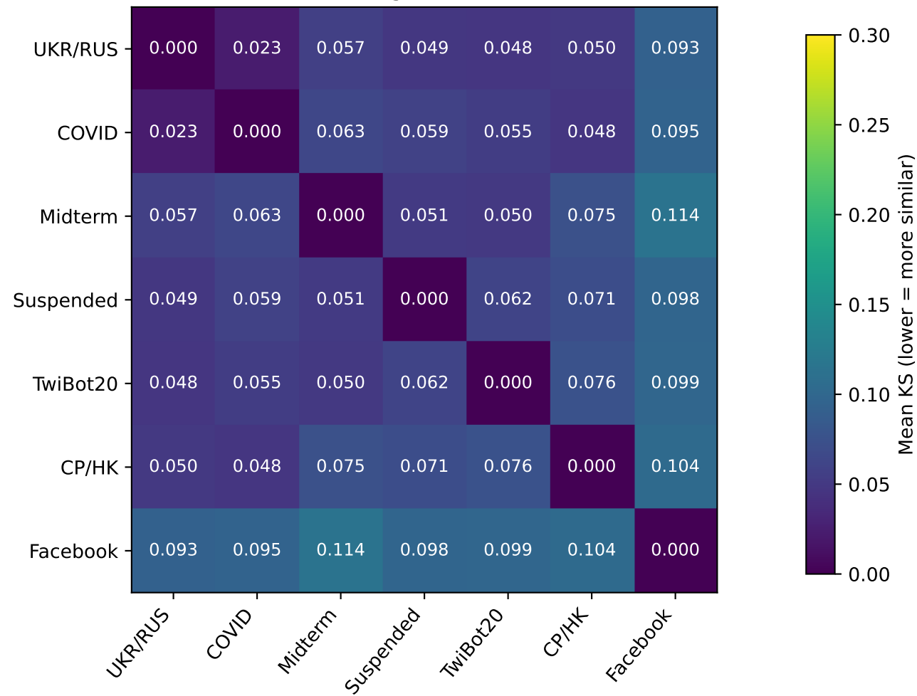
Excluding all-zero rows
