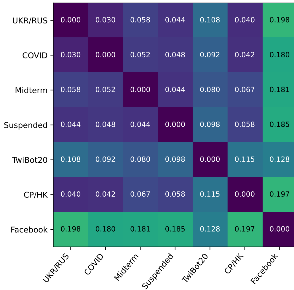
Including all-zero rows
