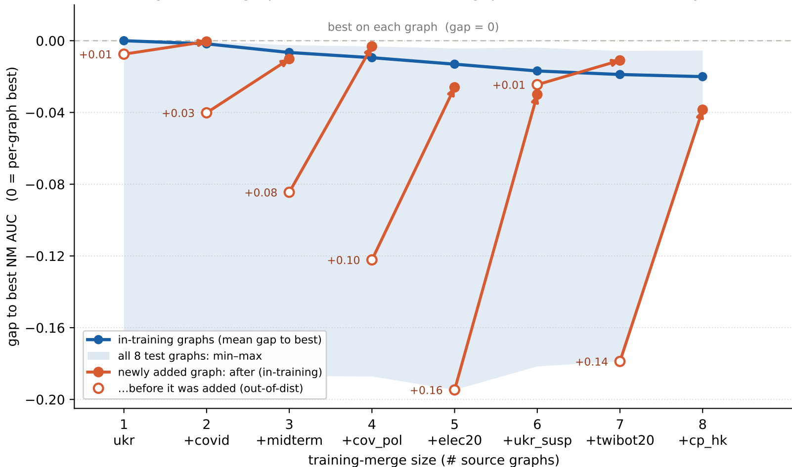
Adding a source graph: newcomers close the gap to best, incumbents stay near it
