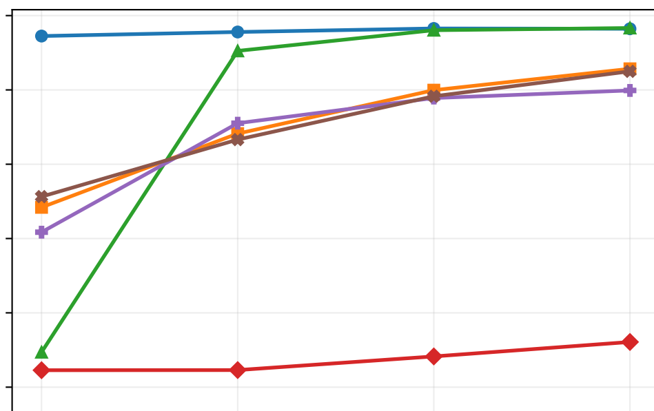
b Election 2020
