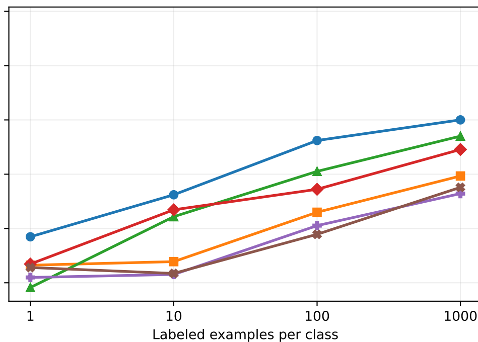
d TwiBot-20
