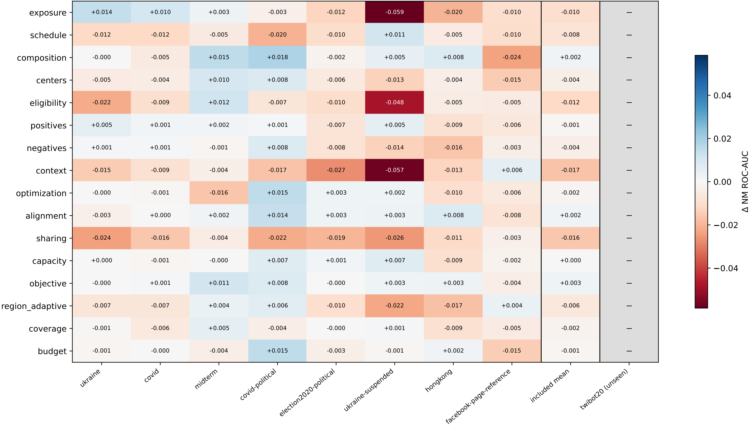
Eight-source endpoint: per-graph NM ROC-AUC difference from baseline
