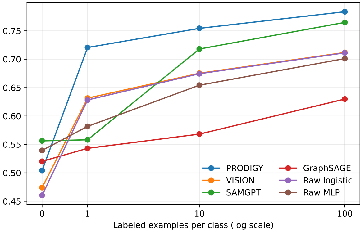
Test ROC-AUC at final scheduled update
