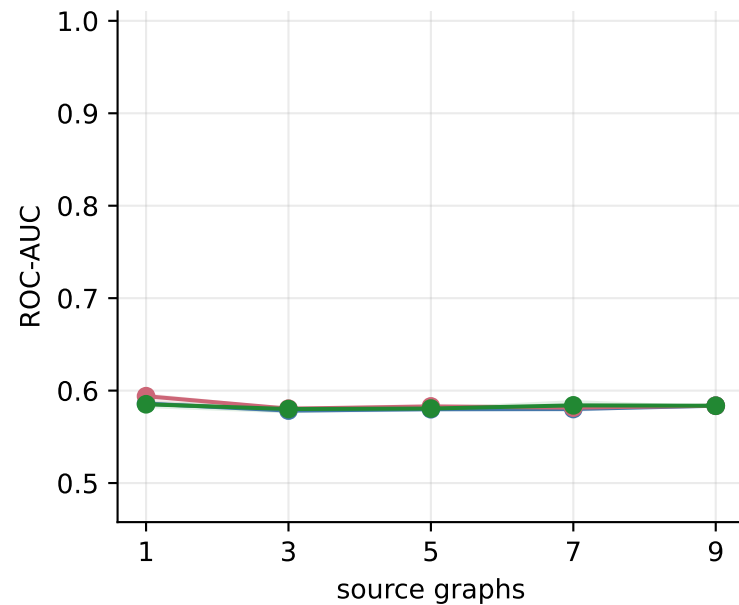
Twibot-20
