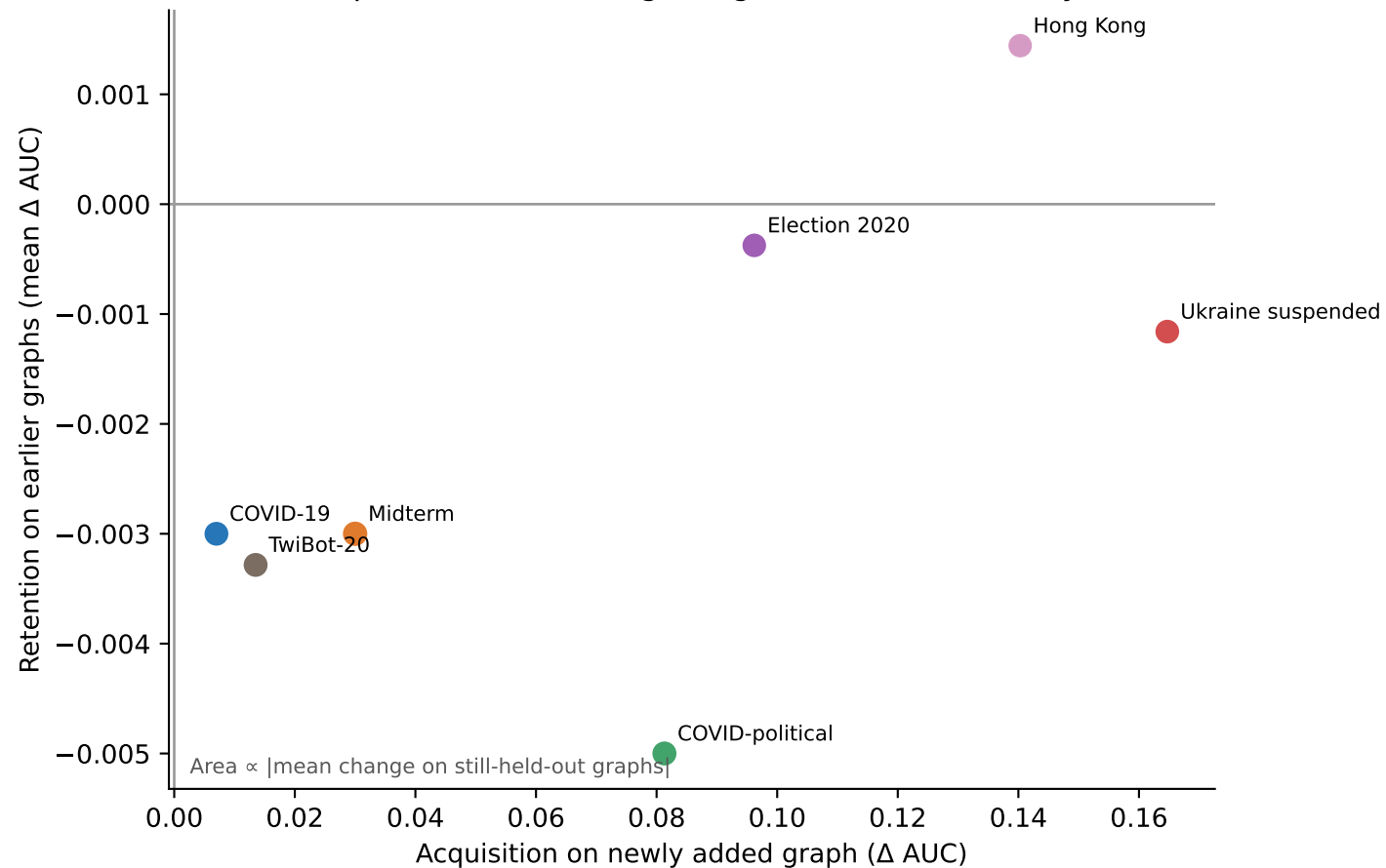
Acquisition versus forgetting at each ladder entry
