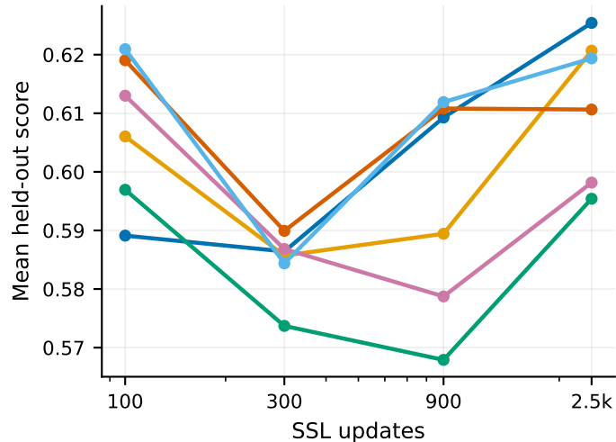
Accuracy
