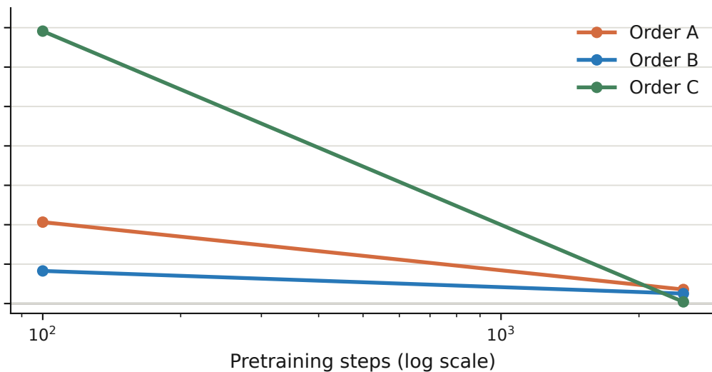
Downstream classification
