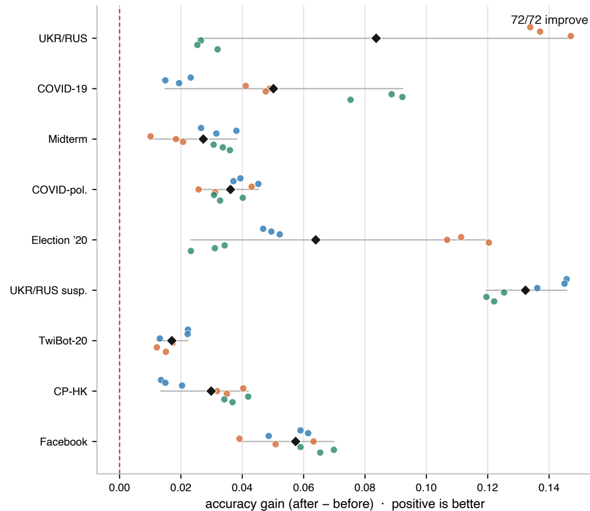
PRODIGY target-entry effects
