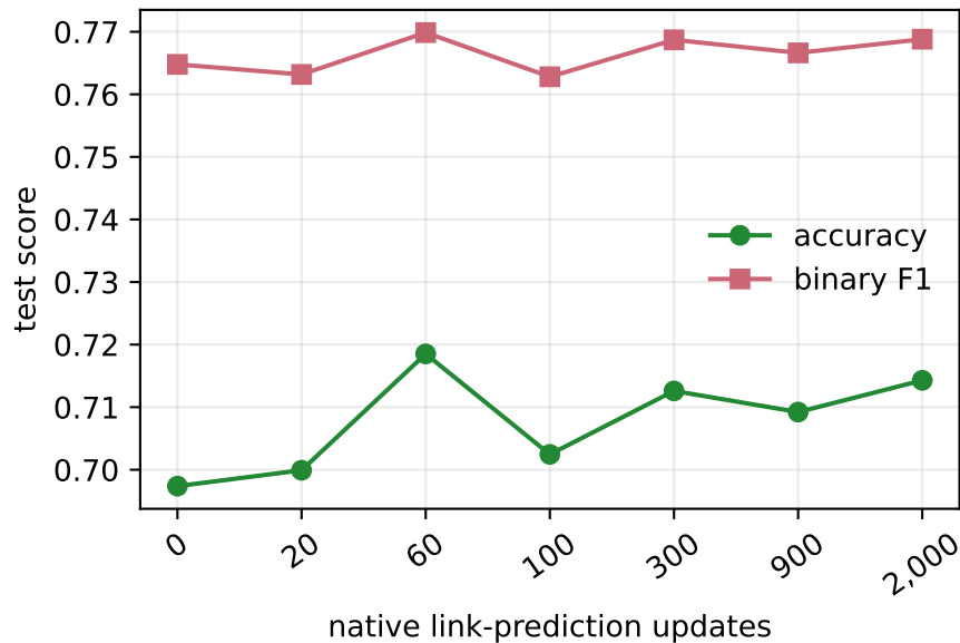
GraphSAGE pilot-v1 → TwiBot CLS saturation full-label official split; one training seed
