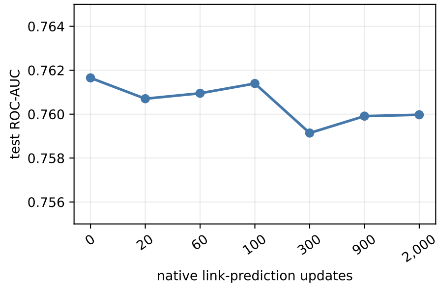
GraphSAGE pilot-v1 → TwiBot CLS saturation full-label official split; one training seed
