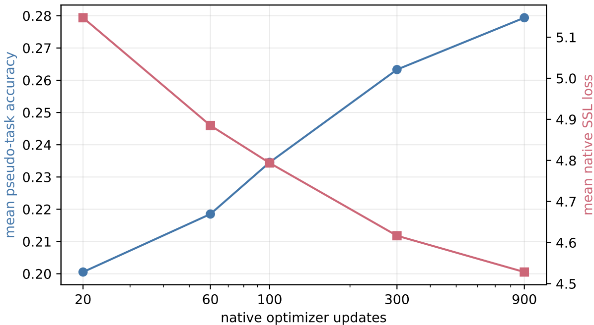
VISION native cross-SSL trajectory (25 source→target pairs)
