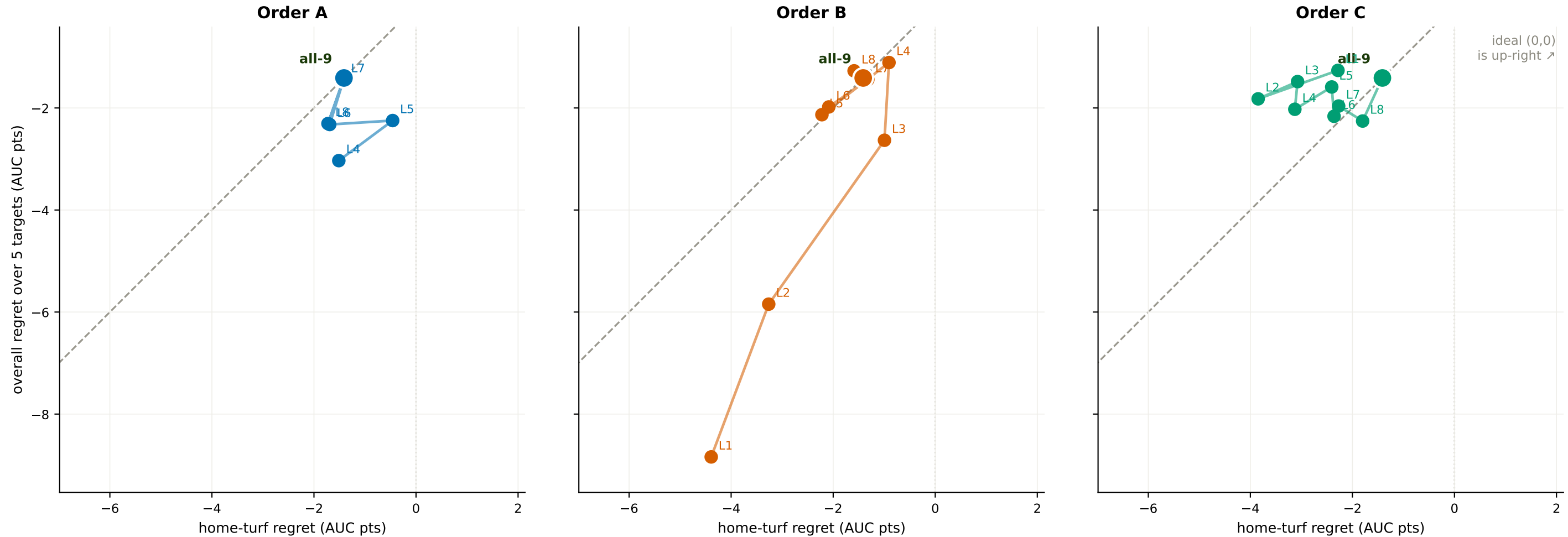
Final-core ladders in regret space — classification (2.5k steps)
