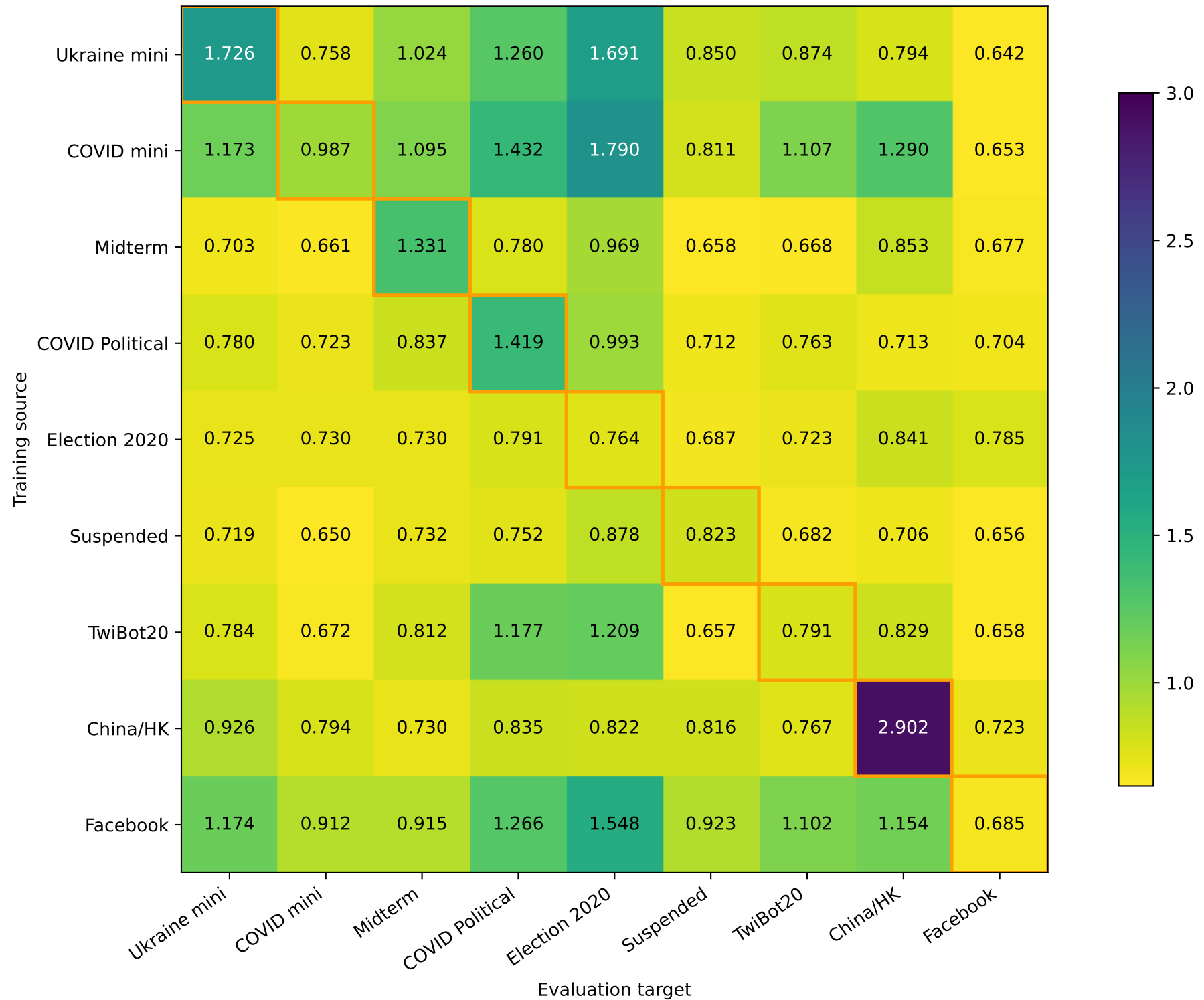
Node + 10-neighbor LP · disjoint context • raw-dot BCE ↓
