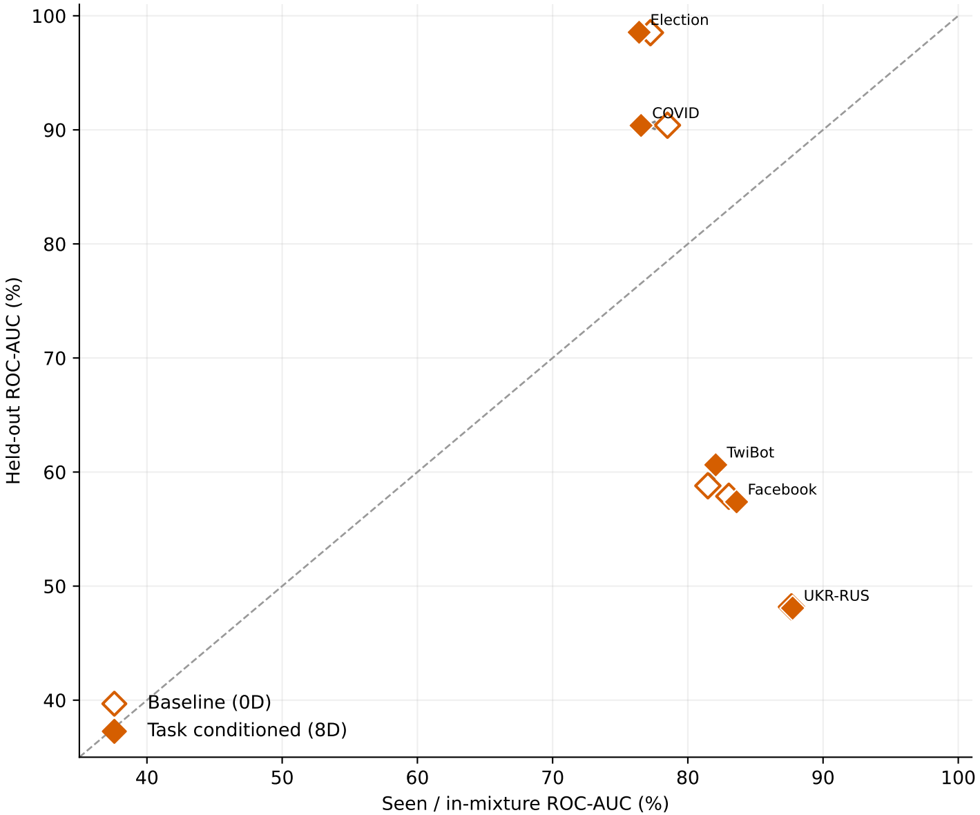
NM+MT 8D task conditioning — ROC-AUC
