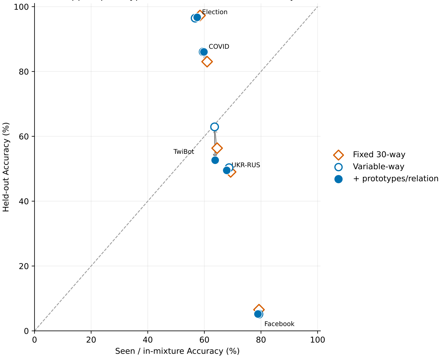
Support prototypes + relation scorer — Accuracy
