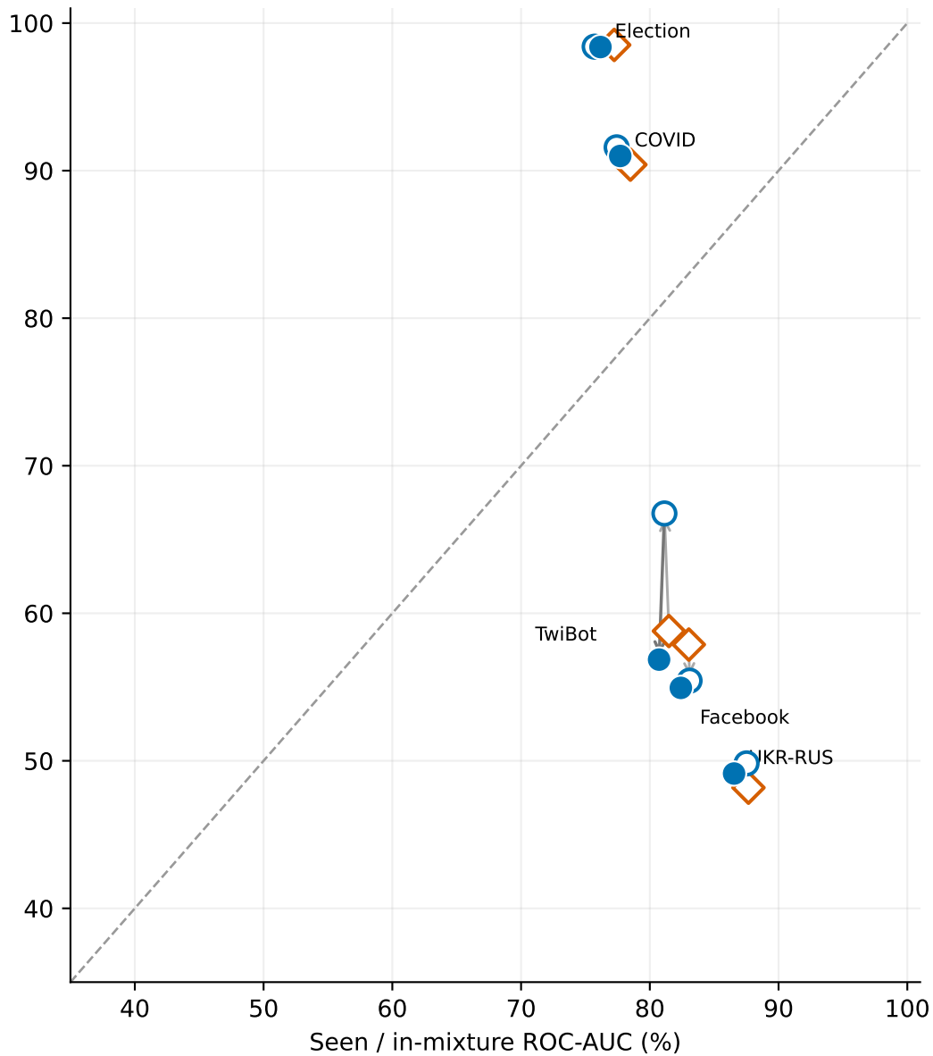
Support prototypes + relation scorer — ROC-AUC
