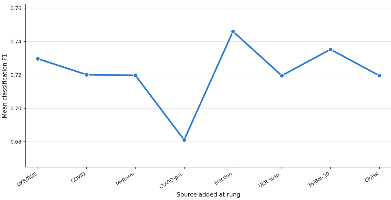
Classification F1 across mixture size
