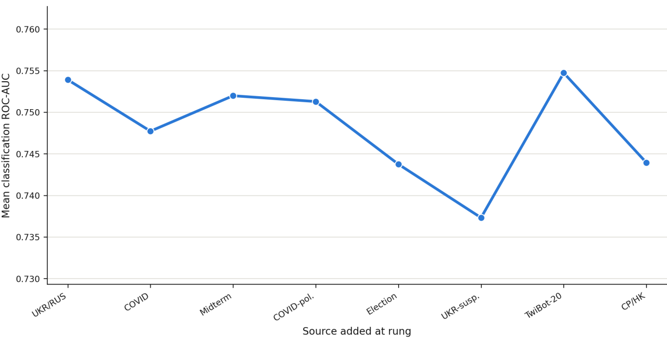
Classification ROC-AUC across mixture size
