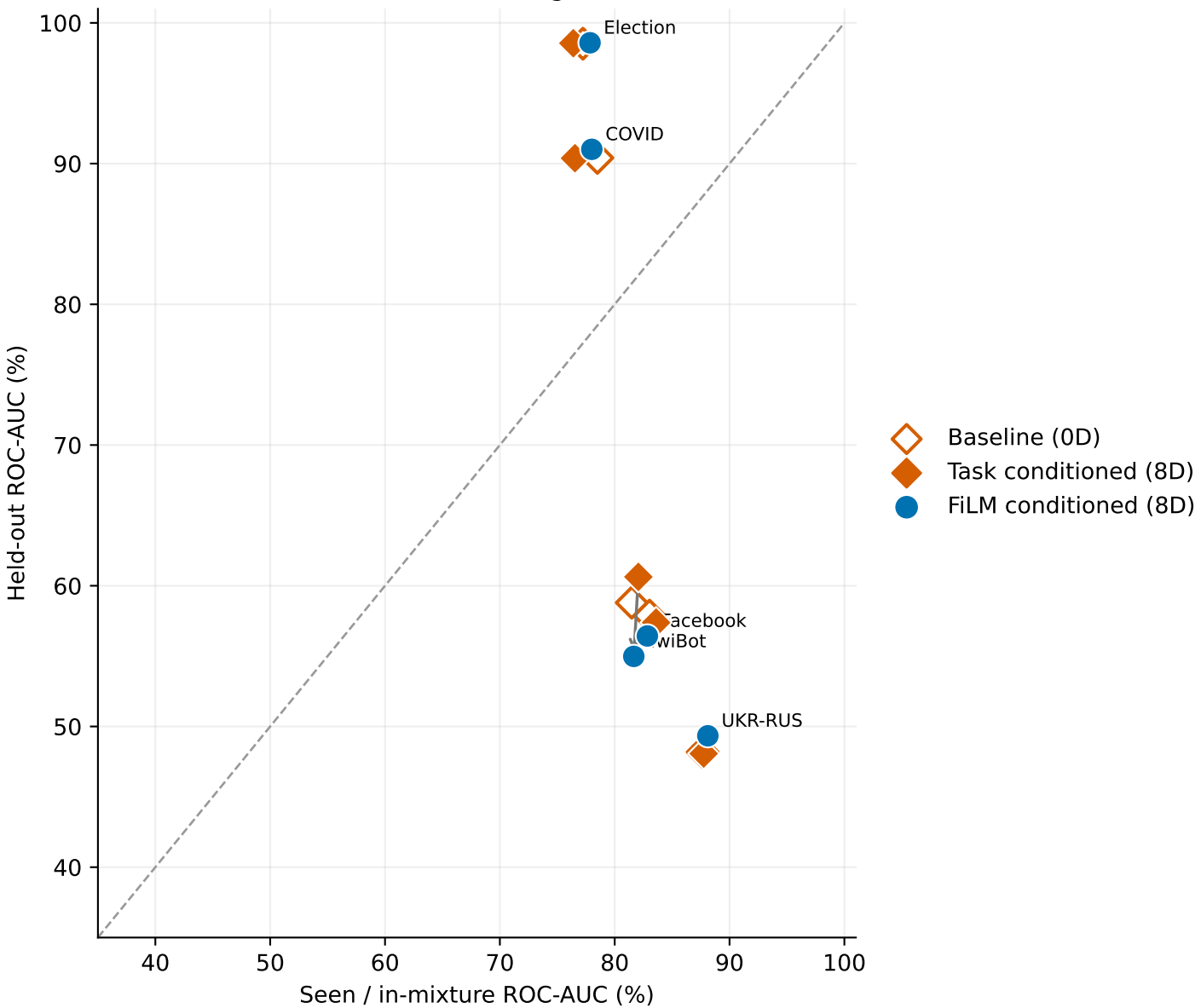
NM+MT task conditioning — ROC-AUC
