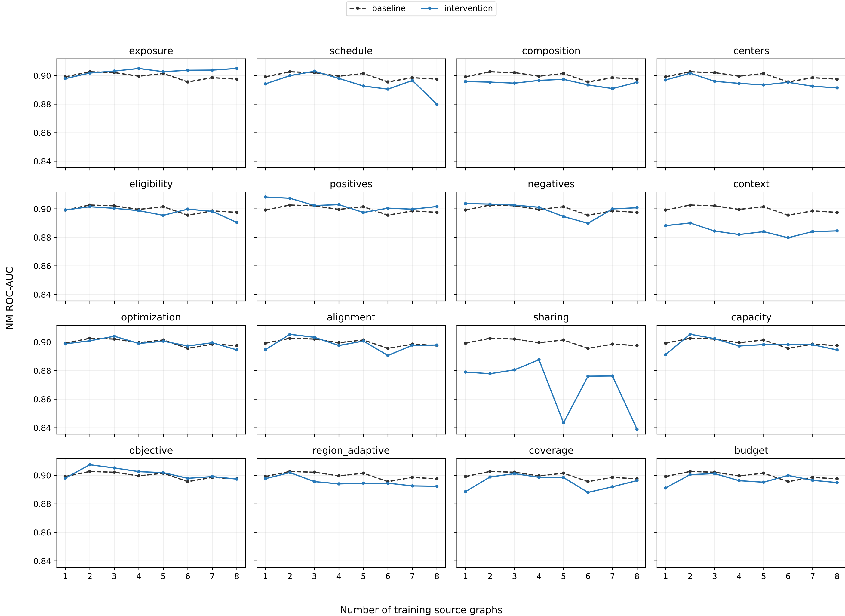
Unseen TwiBot-20: each intervention against baseline (seed 0)
