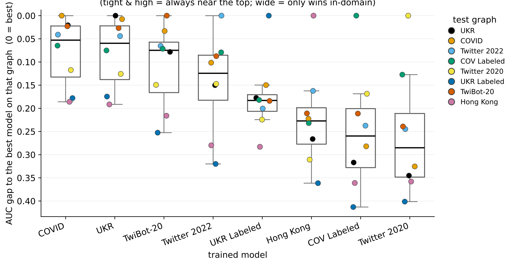
How far each model trails the best on each test graph (tight & high = always near the top; wide = only wins in-domain)
