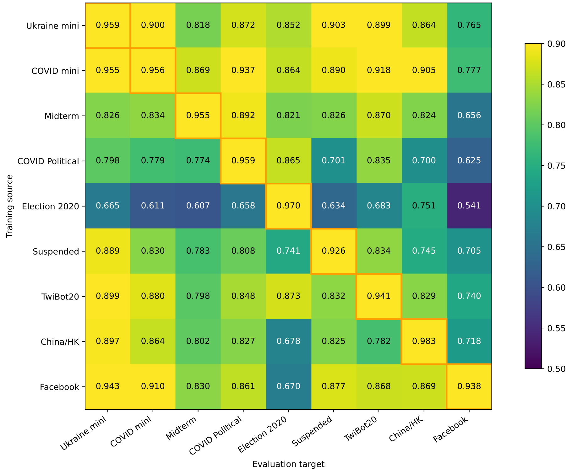
Node + 10-neighbor LP · disjoint context • uniform 1:5 • raw-dot AUC ↑
