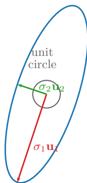
Figure 5: Any matrix maps the unit circle into an ellipse. For \mathbf{A} = \begin{bmatrix} 3 & 0 \\ 4 & 5 \end{bmatrix} , the semi-axes of the resulting ellipse have lengths equal to the singular values \sigma_1 = 3\sqrt{5} and \sigma_2 = \sqrt{5} , oriented along the left singular vectors \mathbf{u}_1 and \mathbf{u}_2 .
