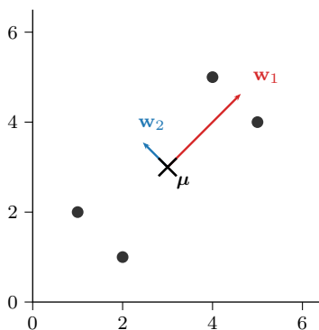
Figure 6: PCA of the four-point dataset in the worked example. The principal components \mathbf{w}_1 and \mathbf{w}_2 (drawn from the data mean and scaled by \sqrt{\lambda_i} ) form an orthogonal coordinate system aligned with the direction of maximum variance.
