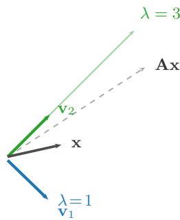
Figure 4: The action of \mathbf{A} = \begin{bmatrix} 2 & 1 \\ 1 & 2 \end{bmatrix} on its eigenvectors: each eigenvector is stretched by its eigenvalue ( \lambda_2 = 3 along \mathbf{v}_2 , \lambda_1 = 1 along \mathbf{v}_1 ) without any change in direction, while a generic vector is both rotated and scaled.
