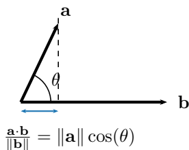
Figure 2: The inner product between vectors \mathbf{a} and \mathbf{b} involves the concept of projecting one vector onto another.
