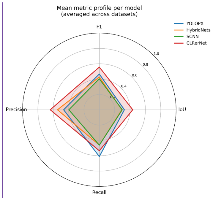
Figure 332. Diagram. Mean metric profile (IoU, F1 Score, Precision, and Recall) for each candidate model, averaged across the four datasets (dataset-normalized). A larger enclosed area indicates stronger overall performance.
