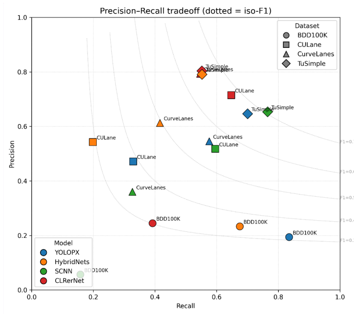
Figure 665. Diagram. Precision-recall trade-off by model and dataset (dotted contours indicate constant-F1 (iso-F1) lines. Points toward the upper right indicate better joint precision and recall).
