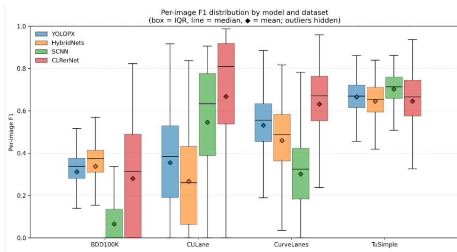
Figure 554. Diagram. Distribution of per-image F1 scores by model and dataset (box = interquartile range, center line = median, diamond = mean; outliers hidden).
