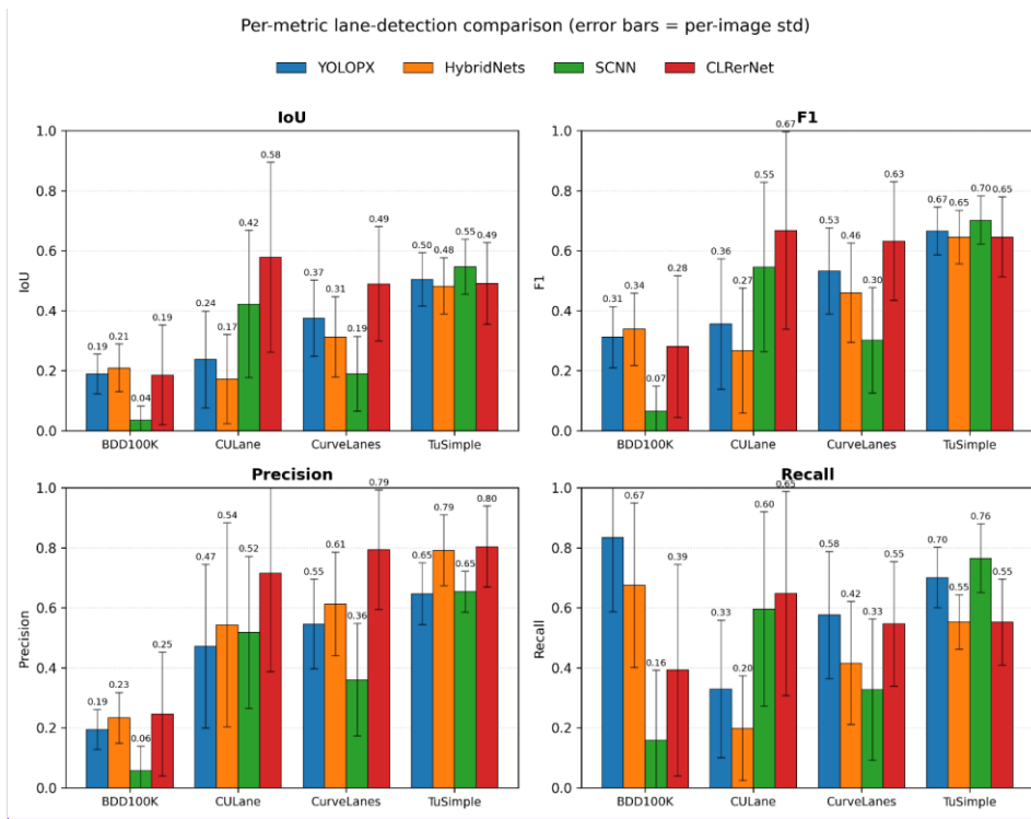
Figure 443. Diagram. Per-dataset comparison of IoU, F1 Score, Precision, and Recall for each candidate model across BDD100K-Lane, CULane, CurveLanes, and TuSimple. Error bars denote per-image standard deviation.
