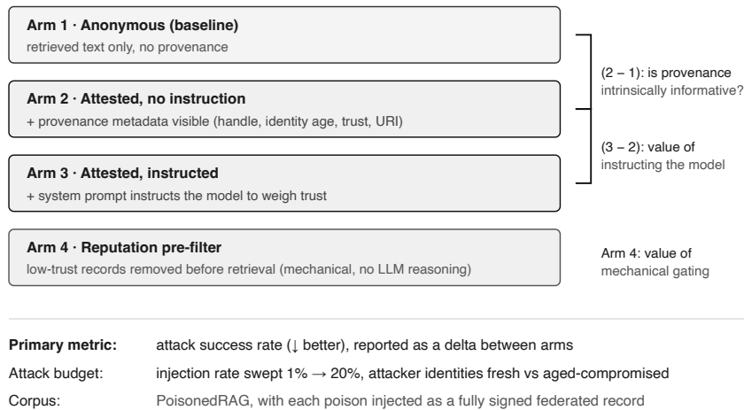
Figure 5. The four-arm provenance-against-poisoning experiment. Each adjacent-arm difference isolates a single causal factor: arm 2 minus arm 1 measures whether provenance is intrinsically informative, arm 3 minus arm 2 measures the value of instructing the model, and arm 4 measures mechanical gating independent of any model reasoning.
