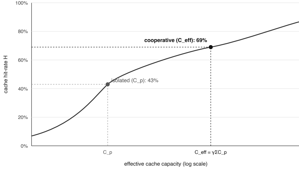
Figure 4. Cooperative caching raises the hit-rate ceiling. Che's approximation evaluated at the pooled effective capacity C_{eff} shifts the operating point along the same saturating curve. The 43% and 69% values are parameter-sensitive model illustrations under one chosen configuration, not measured rates.
