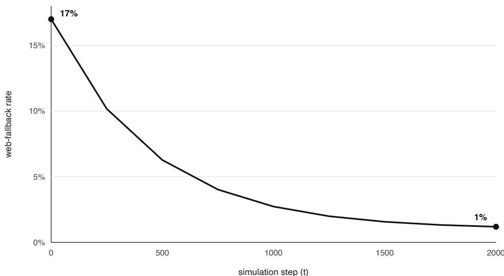
Figure 2. Simulated web-fallback rate over 2,000 steps in AkashikBench-F v1 (10 peers, 20% offline churn, Zipfian demand). The curve is a demonstration, not validated evidence : under v1's boolean-retrieval abstraction the decay is partly true by construction (Sections 5.6 and 7.3). The shape is illustrative of the reported endpoints and negative slope.
