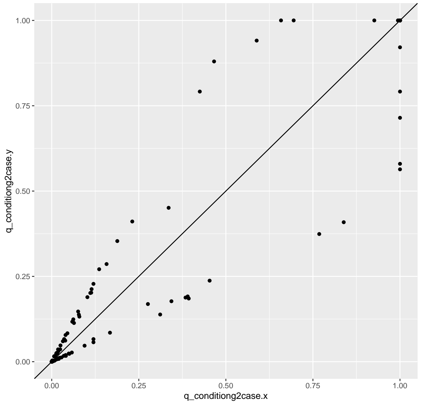
package as-is (x) vs. patched (y)
