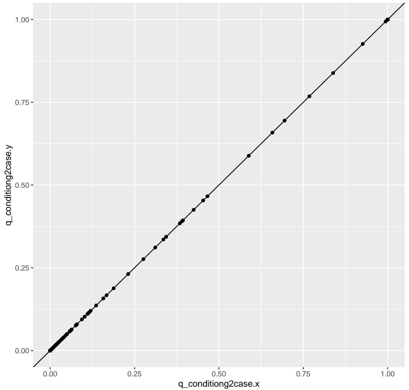
two runs of ANCOMBC2
