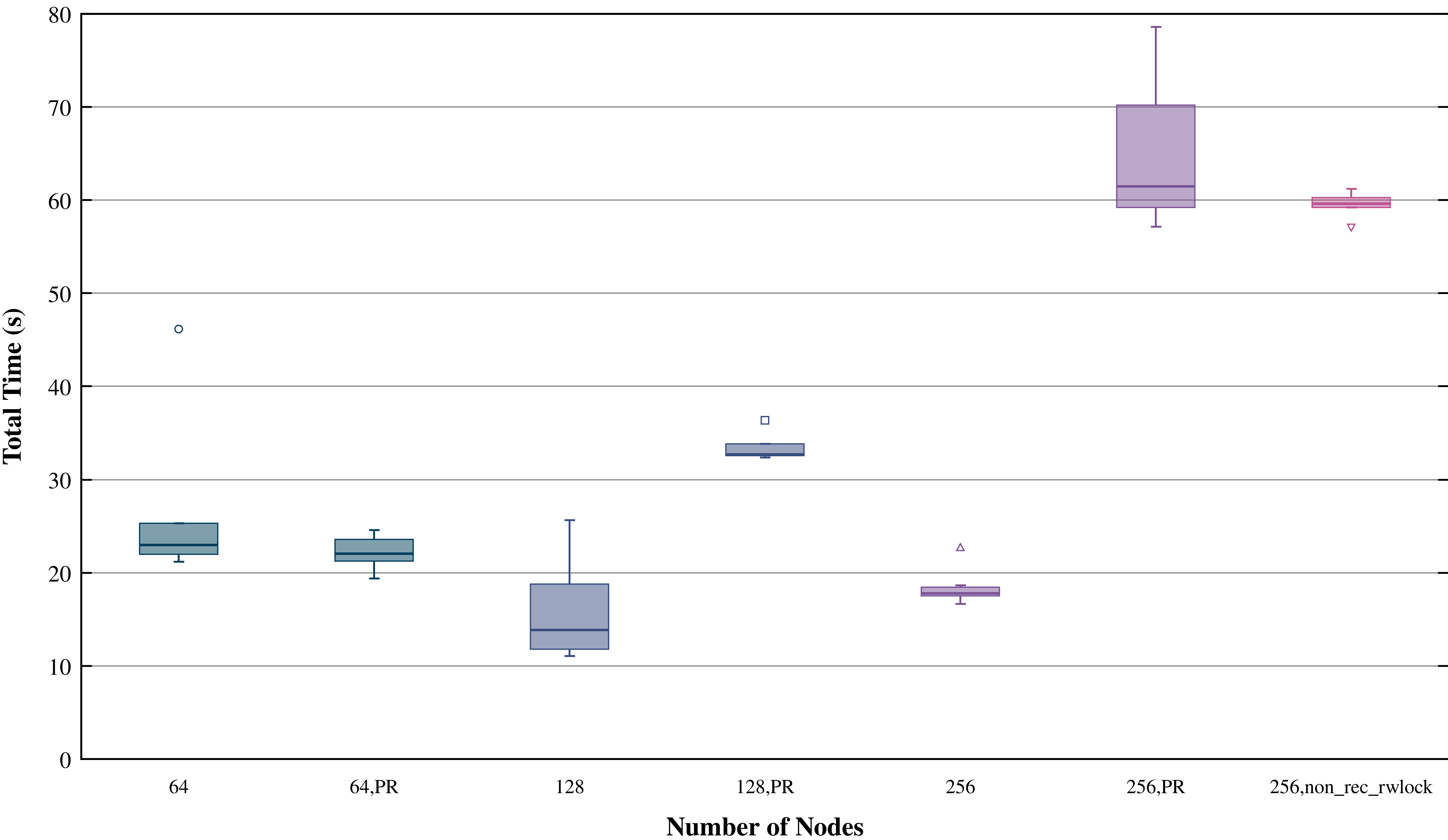
CGNS benchmark, subfiling write/read, Frontier, Node-local Storage
