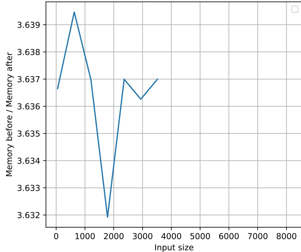
Meta-Llama-3-8B
