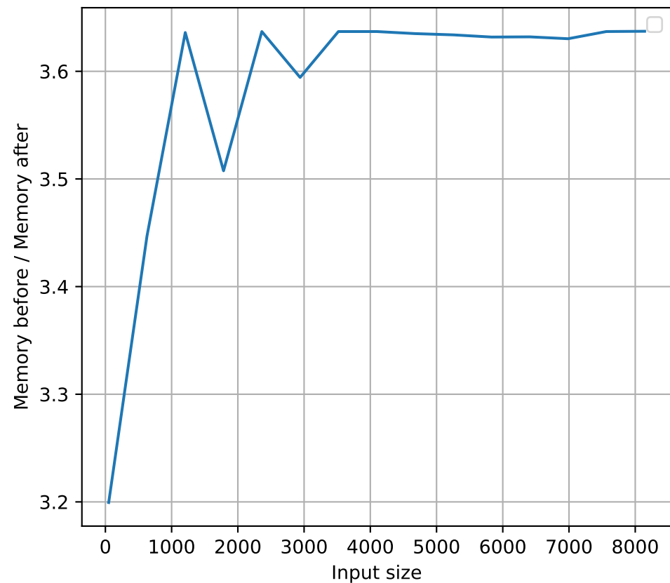
Meta-Llama-3-8B
