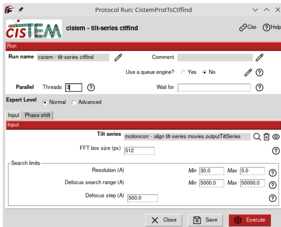
Figure 8: CTFFind protocol.
