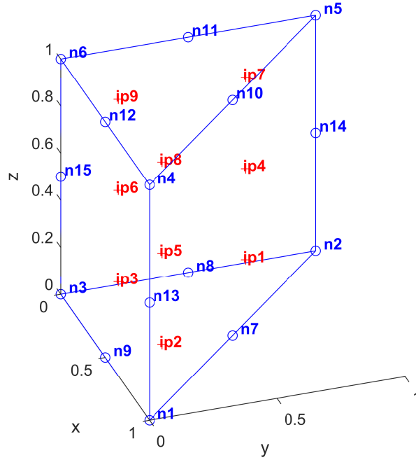
Figure 10: Node (n) and integration point (ip) numbering.
