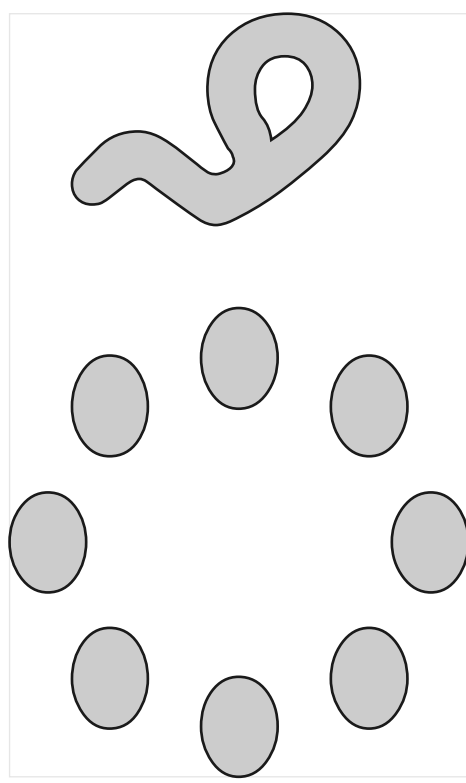
proposed fix
