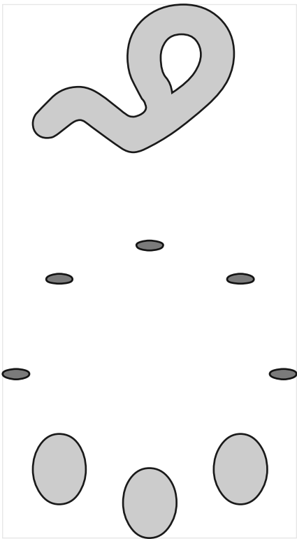
midway interpolation
