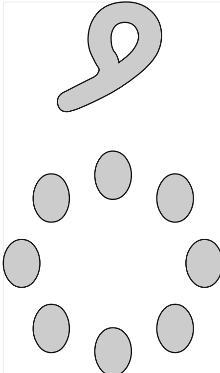
proposed fix
