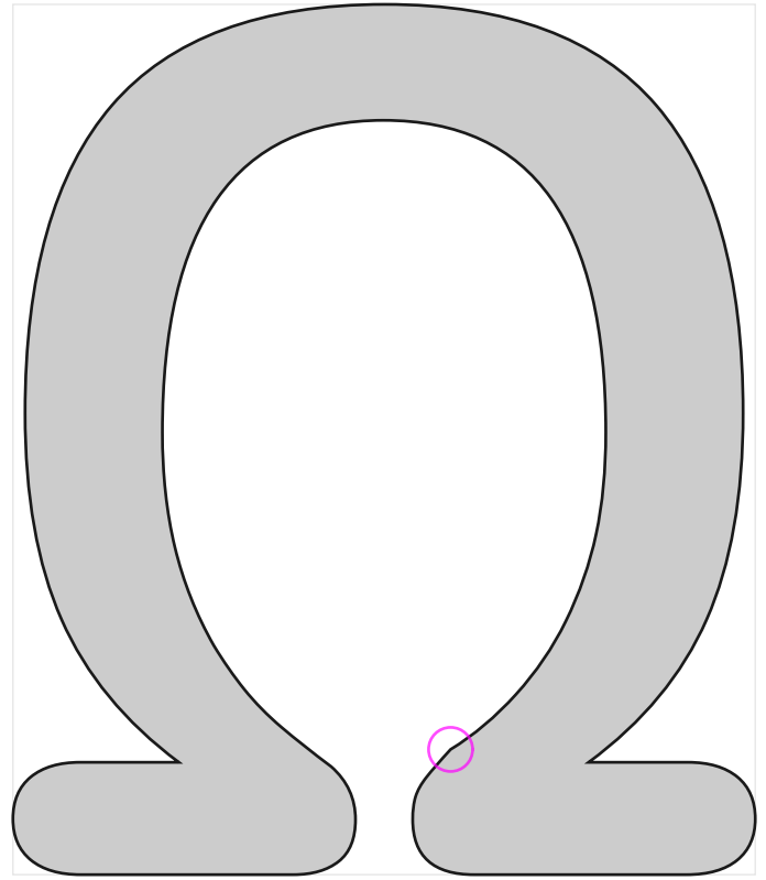
midway interpolation
