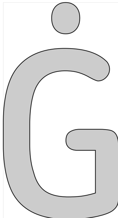
proposed fix
