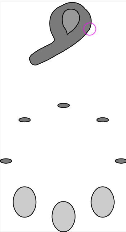
midway interpolation
