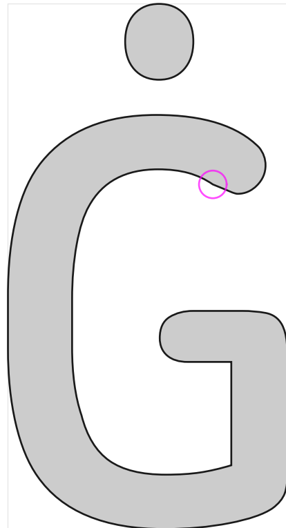
midway interpolation
