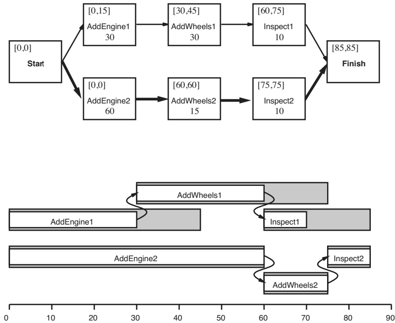
Figure 11.2 Top: a representation of the temporal constraints for the job-shop scheduling problem of Figure 11.1. The duration of each action is given at the bottom of each rectangle. In solving the problem, we compute the earliest and latest start times as the pair [ES, LS] , displayed in the upper left. The difference between these two numbers is the slack of an action; actions with zero slack are on the critical path, shown with bold arrows. Bottom: the same solution shown as a timeline. Grey rectangles represent time intervals during which an action may be executed, provided that the ordering constraints are respected. The unoccupied portion of a gray rectangle indicates the slack.
