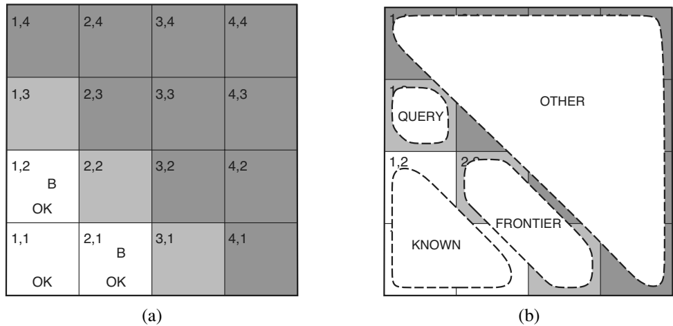
Figure 13.5 (a) After finding a breeze in both [1,2] and [2,1], the agent is stuck—there is no safe place to explore. (b) Division of the squares into Known , Frontier , and Other , for a query about [1,3].
