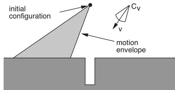
Figure 25.20 The first motion command and the resulting envelope of possible robot motions. No matter what the error, we know the final configuration will be to the left of the hole.
