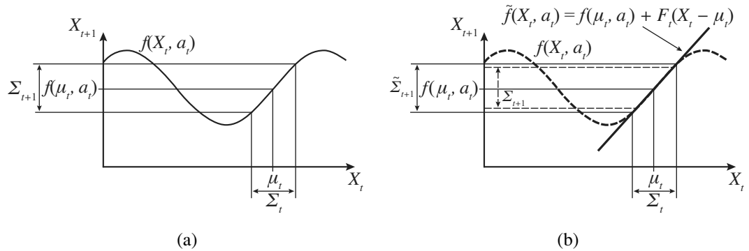
Figure 25.11 One-dimensional illustration of a linearized motion model: (a) The function f , and the projection of a mean \mu_t and a covariance interval (based on \Sigma_t ) into time t + 1 . (b) The linearized version is the tangent of f at \mu_t . The projection of the mean \mu_t is correct. However, the projected covariance \tilde{\Sigma}_{t+1} differs from \Sigma_{t+1} .
