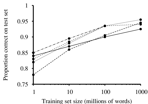
Figure 18.37 Learning curves for five learning algorithms on a common task. Note that there appears to be more room for improvement in the horizontal direction (more training data) than in the vertical direction (different machine learning algorithm). Adapted from Banko and Brill (2001).
