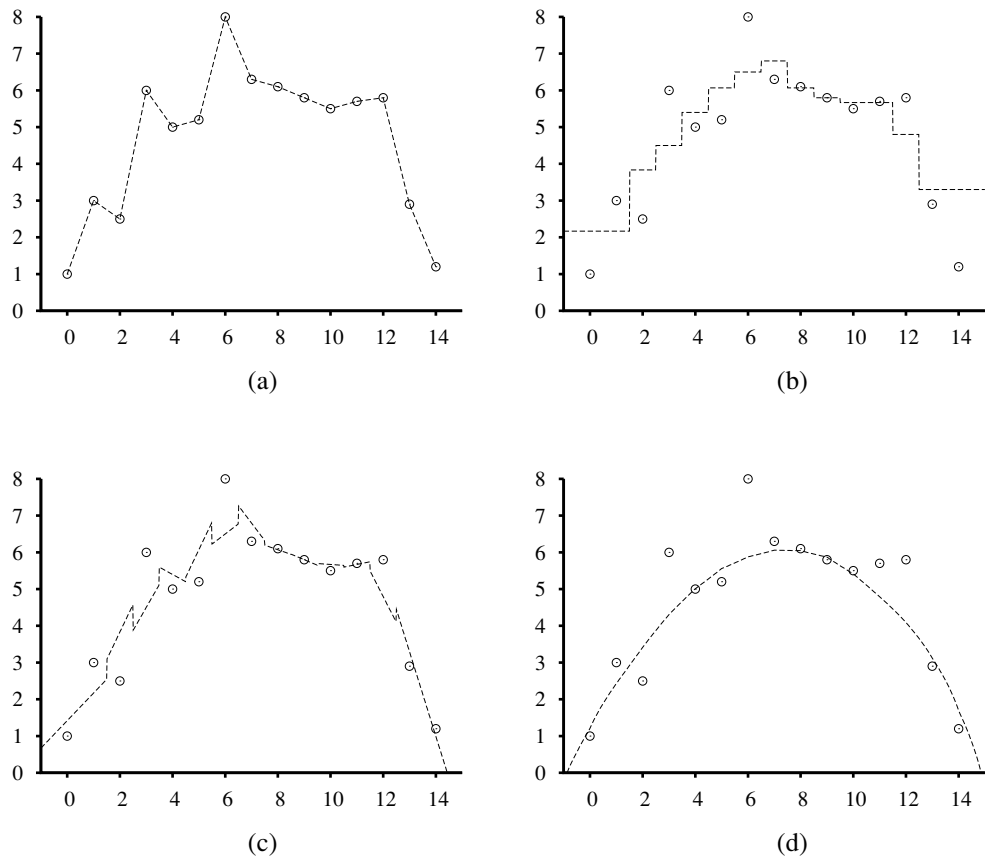
Figure 18.28 Nonparametric regression models: (a) connect the dots, (b) 3-nearest neighbors average, (c) 3-nearest-neighbor linear regression, (d) locally weighted regression with a quadratic kernel of width k = 10 .
