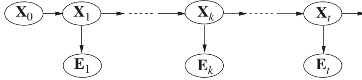
Figure 15.3 Smoothing computes \mathbf{P}(\mathbf{X}_k | \mathbf{e}_{1:t}) , the posterior distribution of the state at some past time k given a complete sequence of observations from 1 to t .
