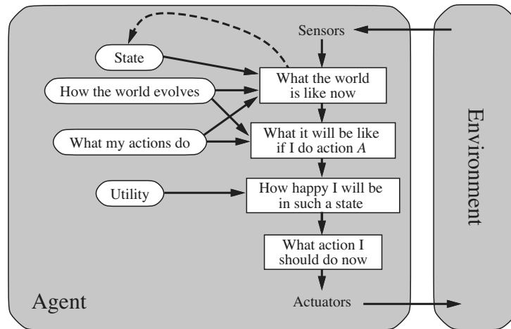
Figure 27.1 A model-based, utility-based agent, as first presented in Figure 2.14.
