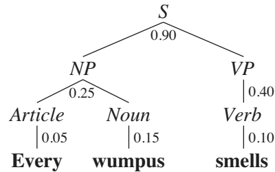
Figure 23.3 Parse tree for the sentence “Every wumpus smells” according to the grammar \mathcal{E}_0 . Each interior node of the tree is labeled with its probability. The probability of the tree as a whole is 0.9 \times 0.25 \times 0.05 \times 0.15 \times 0.40 \times 0.10 = 0.0000675 . Since this tree is the only parse of the sentence, that number is also the probability of the sentence. The tree can also be written in linear form as [S [NP [Article \textbf{every}] [Noun \textbf{wumpus}]] [VP [Verb \textbf{smells}]]] .
