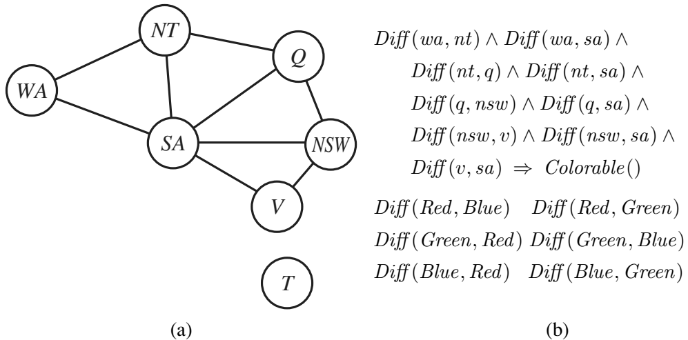
Figure 9.5 (a) Constraint graph for coloring the map of Australia. (b) The map-coloring CSP expressed as a single definite clause. Each map region is represented as a variable whose value can be one of the constants Red , Green or Blue .
