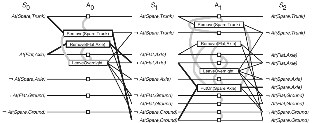
Figure 10.10 The planning graph for the spare tire problem after expansion to level S_2 . Mutex links are shown as gray lines. Not all links are shown, because the graph would be too cluttered if we showed them all. The solution is indicated by bold lines and outlines.
