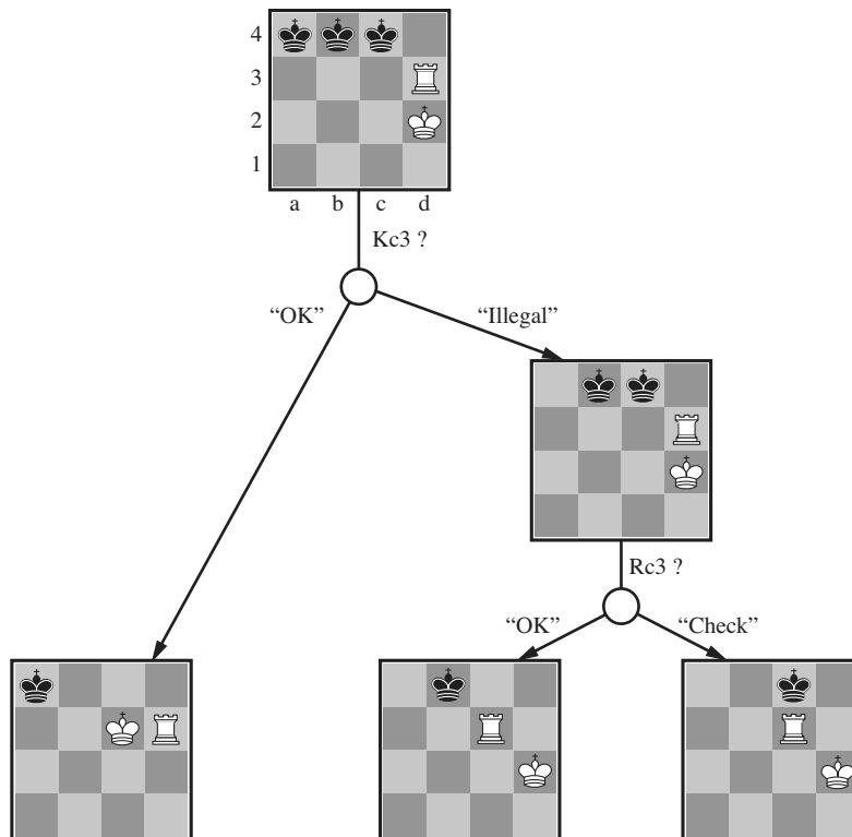
Figure 5.13 Part of a guaranteed checkmate in the KKR endgame, shown on a reduced board. In the initial belief state, Black’s king is in one of three possible locations. By a combination of probing moves, the strategy narrows this down to one. Completion of the checkmate is left as an exercise.
