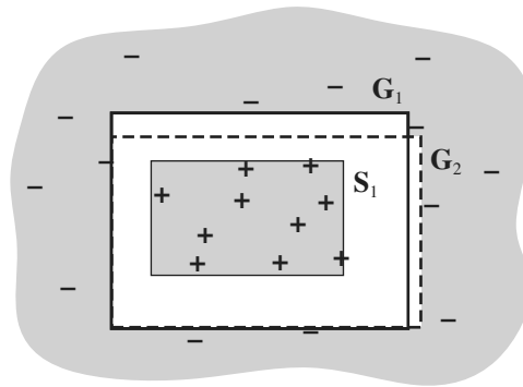
Figure 19.5 The extensions of the members of G and S . No known examples lie in between the two sets of boundaries.
