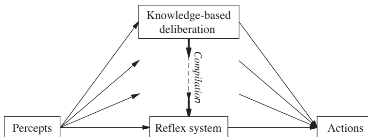
Figure 27.2 Compilation serves to convert deliberative decision making into more efficient, reflexive mechanisms.
