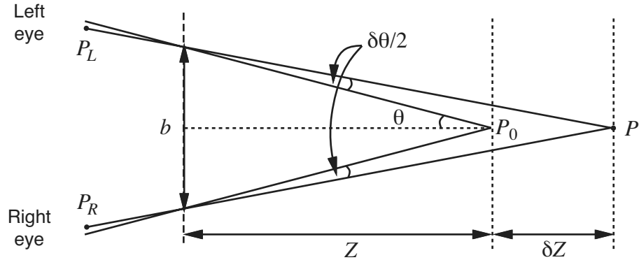
Figure 24.17 The relation between disparity and depth in stereopsis. The centers of projection of the two eyes are b apart, and the optical axes intersect at the fixation point P_0 . The point P in the scene projects to points P_L and P_R in the two eyes. In angular terms, the disparity between these is \delta\theta . See text.
