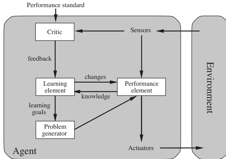
Figure 2.15 A general learning agent.
