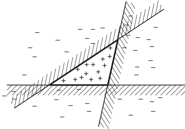
Figure 18.32 Illustration of the increased expressive power obtained by ensemble learning. We take three linear threshold hypotheses, each of which classifies positively on the unshaded side, and classify as positive any example classified positively by all three. The resulting triangular region is a hypothesis not expressible in the original hypothesis space.
