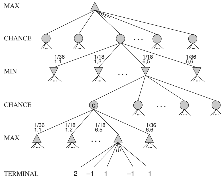
Figure 5.11 Schematic game tree for a backgammon position.
