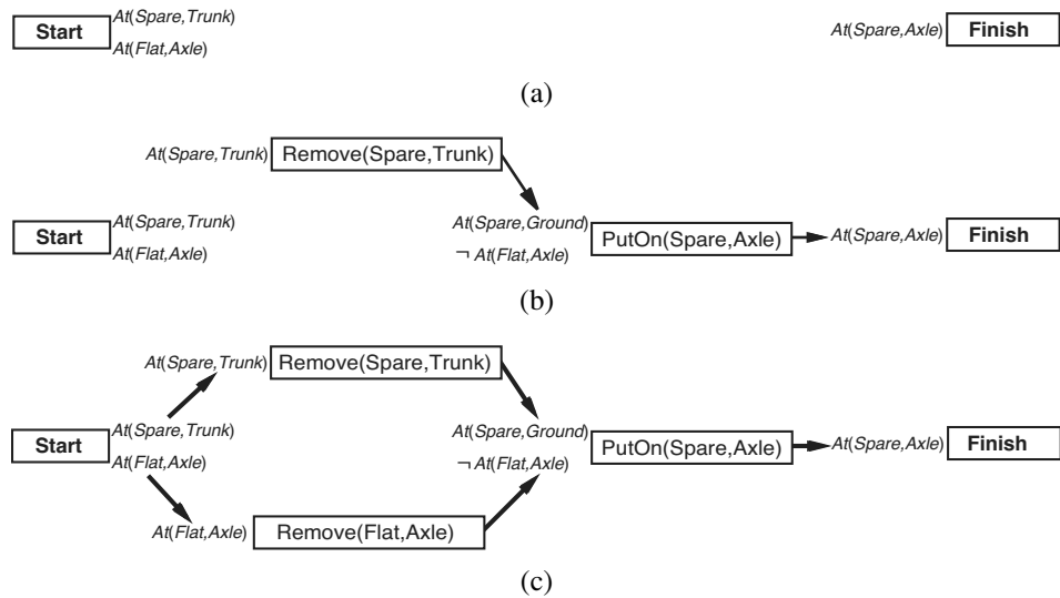
Figure 10.13 (a) the tire problem expressed as an empty plan. (b) an incomplete partially ordered plan for the tire problem. Boxes represent actions and arrows indicate that one action must occur before another. (c) a complete partially-ordered solution.
