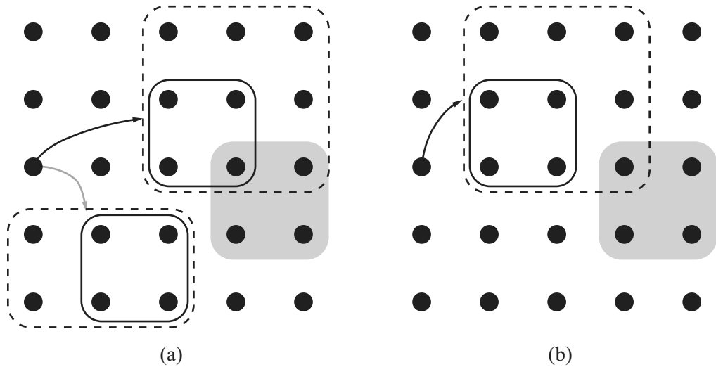
Figure 11.7 Goal achievement for high-level plans with approximate descriptions. The set of goal states is shaded. For each plan, the pessimistic (solid lines) and optimistic (dashed lines) reachable sets are shown. (a) The plan indicated by the black arrow definitely achieves the goal, while the plan indicated by the gray arrow definitely doesn't. (b) A plan that would need to be refined further to determine if it really does achieve the goal.
