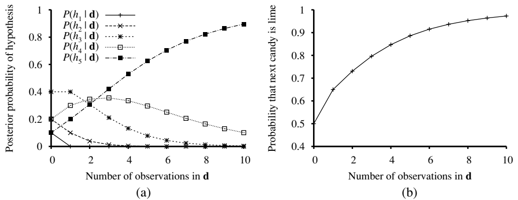
Figure 20.1 (a) Posterior probabilities P(h_i | d_1, \dots, d_N) from Equation (20.1). The number of observations N ranges from 1 to 10, and each observation is of a lime candy. (b) Bayesian prediction P(d_{N+1} = \text{lime} | d_1, \dots, d_N) from Equation (20.2).
