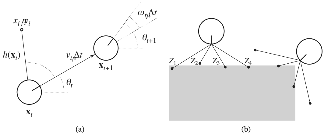
Figure 25.8 (a) A simplified kinematic model of a mobile robot. The robot is shown as a circle with an interior line marking the forward direction. The state \mathbf{x}_t consists of the (x_t, y_t) position (shown implicitly) and the orientation \theta_t . The new state \mathbf{x}_{t+1} is obtained by an update in position of v_t \Delta t and in orientation of \omega_t \Delta t . Also shown is a landmark at (x_i, y_i) observed at time t . (b) The range-scan sensor model. Two possible robot poses are shown for a given range scan (z_1, z_2, z_3, z_4) . It is much more likely that the pose on the left generated the range scan than the pose on the right.
