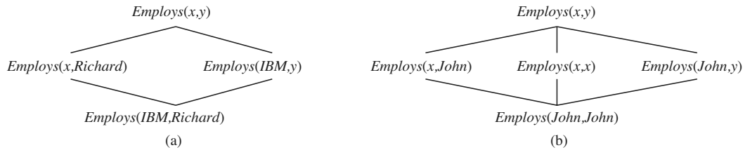
Figure 9.2 (a) The subsumption lattice whose lowest node is Employes(IBM, Richard) . (b) The subsumption lattice for the sentence Employes(John, John) .
