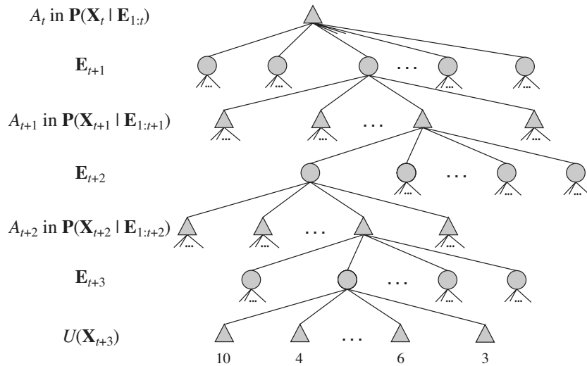
Figure 17.11 Part of the look-ahead solution of the DDN in Figure 17.10. Each decision will be taken in the belief state indicated.
