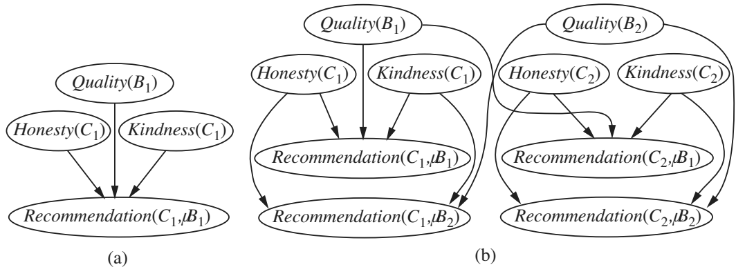
Figure 14.17 (a) Bayes net for a single customer C_1 recommending a single book B_1 . Honest(C_1) is Boolean, while the other variables have integer values from 1 to 5. (b) Bayes net with two customers and two books.
