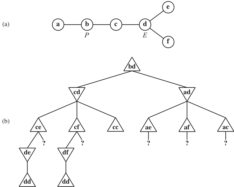
Figure 5.16 (a) A map where the cost of every edge is 1. Initially the pursuer P is at node b and the evader E is at node d . (b) A partial game tree for this map. Each node is labeled with the P, E positions. P moves first. Branches marked “?” have yet to be explored.
