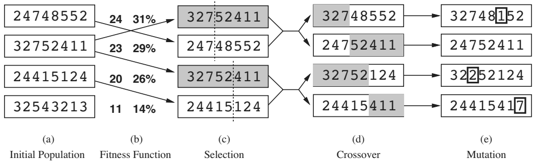
Figure 4.6 The genetic algorithm, illustrated for digit strings representing 8-queens states. The initial population in (a) is ranked by the fitness function in (b), resulting in pairs for mating in (c). They produce offspring in (d), which are subject to mutation in (e).
