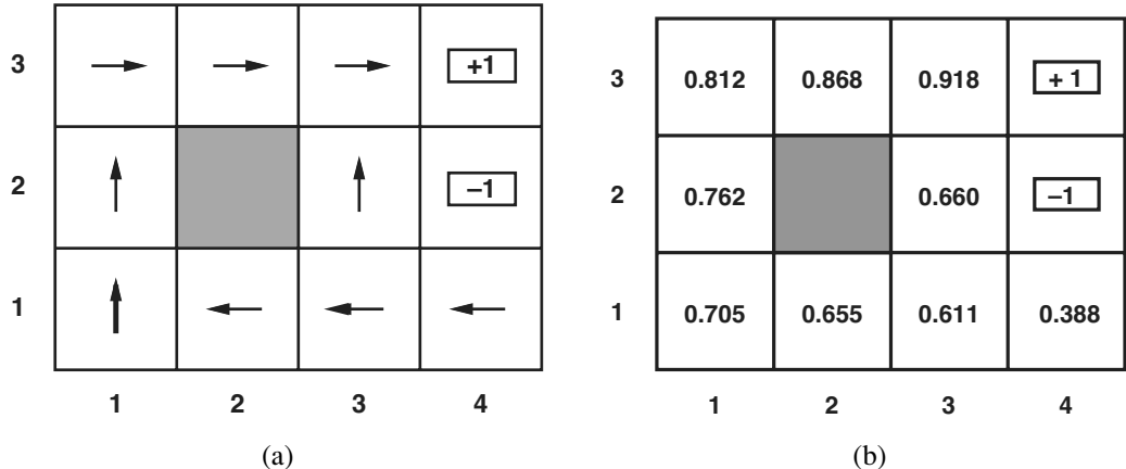
Figure 21.1 (a) A policy \pi for the 4 \times 3 world; this policy happens to be optimal with rewards of R(s) = -0.04 in the nonterminal states and no discounting. (b) The utilities of the states in the 4 \times 3 world, given policy \pi .
