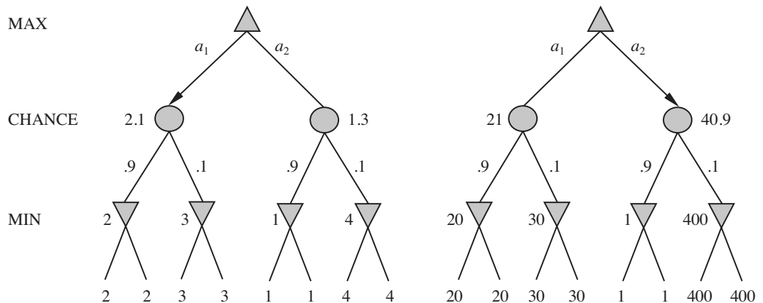
Figure 5.12 An order-preserving transformation on leaf values changes the best move.
