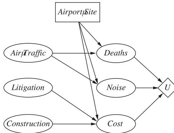
Figure 16.6 A simple decision network for the airport-siting problem.
