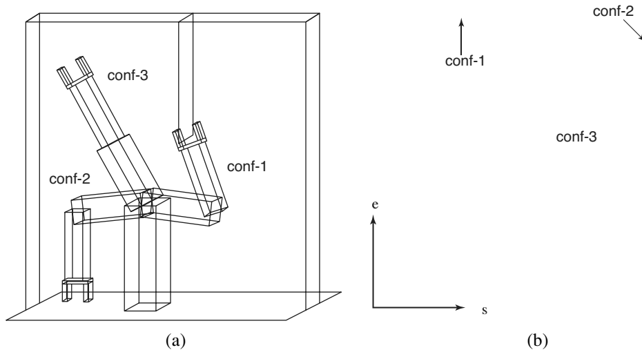
Figure 25.15 Three robot configurations, shown in workspace and configuration space.
