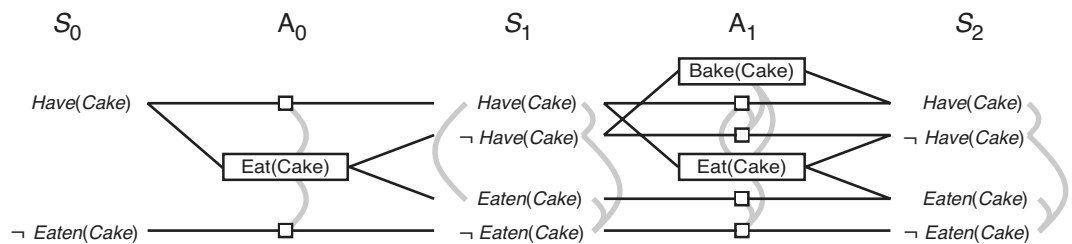
Figure 10.8 The planning graph for the “have cake and eat cake too” problem up to level S_2 . Rectangles indicate actions (small squares indicate persistence actions), and straight lines indicate preconditions and effects. Mutex links are shown as curved gray lines. Not all mutex links are shown, because the graph would be too cluttered. In general, if two literals are mutex at S_i , then the persistence actions for those literals will be mutex at A_i and we need not draw that mutex link.
