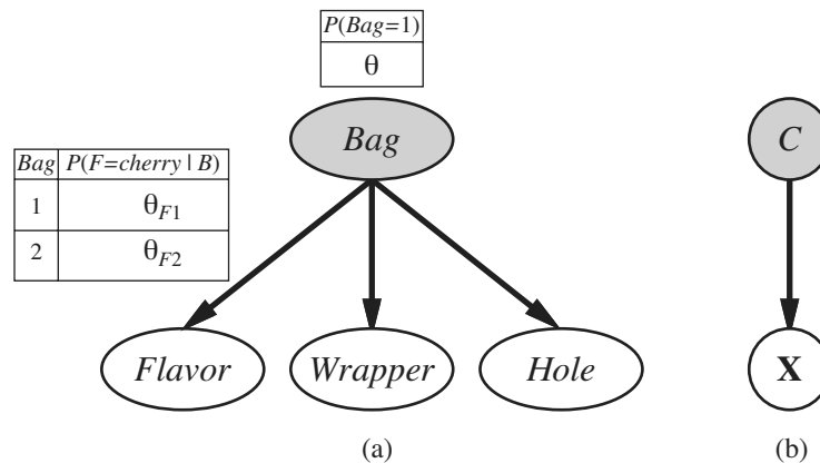
Figure 20.13 (a) A mixture model for candy. The proportions of different flavors, wrappers, presence of holes depend on the bag, which is not observed. (b) Bayesian network for a Gaussian mixture. The mean and covariance of the observable variables \mathbf{X} depend on the component C .
