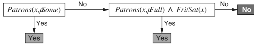
Figure 18.10 A decision list for the restaurant problem.
