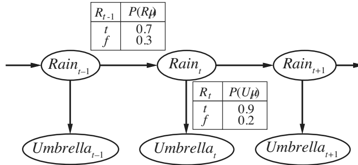
Figure 15.2 Bayesian network structure and conditional distributions describing the umbrella world. The transition model is P(\text{Rain}_t | \text{Rain}_{t-1}) and the sensor model is P(\text{Umbrella}_t | \text{Rain}_t) .
