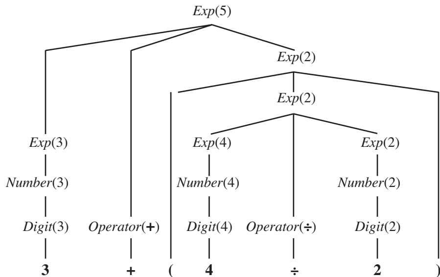
Figure 23.9 Parse tree with semantic interpretations for the string “ 3 + (4 \div 2) ”.
