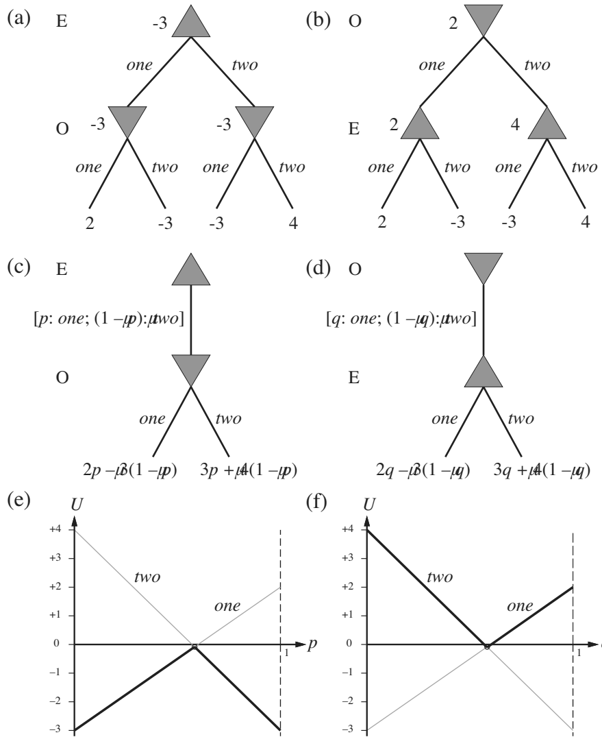
Figure 17.12 (a) and (b): Minimax game trees for two-finger Morra if the players take turns playing pure strategies. (c) and (d): Parameterized game trees where the first player plays a mixed strategy. The payoffs depend on the probability parameter ( p or q ) in the mixed strategy. (e) and (f): For any particular value of the probability parameter, the second player will choose the “better” of the two actions, so the value of the first player’s mixed strategy is given by the heavy lines. The first player will choose the probability parameter for the mixed strategy at the intersection point.
