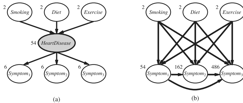
Figure 20.10 (a) A simple diagnostic network for heart disease, which is assumed to be a hidden variable. Each variable has three possible values and is labeled with the number of independent parameters in its conditional distribution; the total number is 78. (b) The equivalent network with HeartDisease removed. Note that the symptom variables are no longer conditionally independent given their parents. This network requires 708 parameters.
