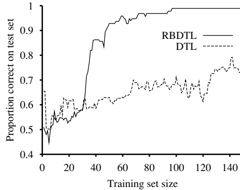
Figure 19.9 A performance comparison between DECISION-TREE-LEARNING and RBDTL on randomly generated data for a target function that depends on only 5 of 16 attributes.
