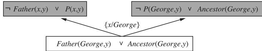
Figure 19.14 An inverse resolution step that generates a new predicate P .
