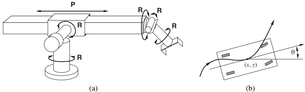
Figure 25.4 (a) The Stanford Manipulator, an early robot arm with five revolute joints (R) and one prismatic joint (P), for a total of six degrees of freedom. (b) Motion of a nonholonomic four-wheeled vehicle with front-wheel steering.
