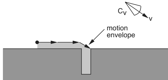
Figure 25.21 The second motion command and the envelope of possible motions. Even with error, we will eventually get into the hole.
