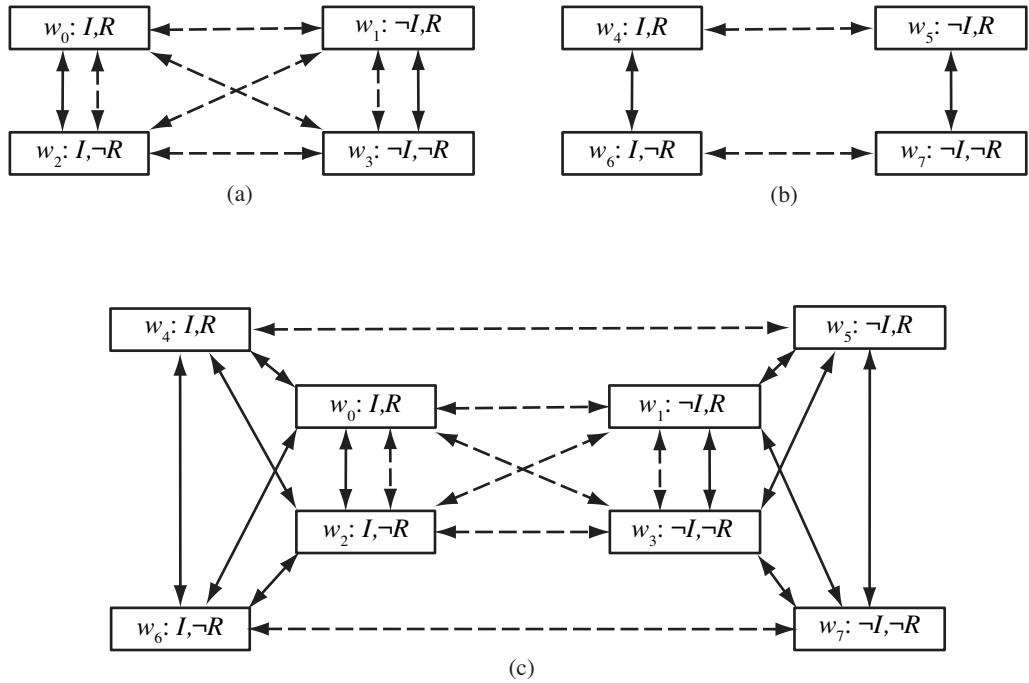
Figure 12.4 Possible worlds with accessibility relations \mathbf{K}_{Superman} (solid arrows) and \mathbf{K}_{Lois} (dotted arrows). The proposition R means “the weather report for tomorrow is rain” and I means “Superman’s secret identity is Clark Kent.” All worlds are accessible to themselves; the arrows from a world to itself are not shown.
