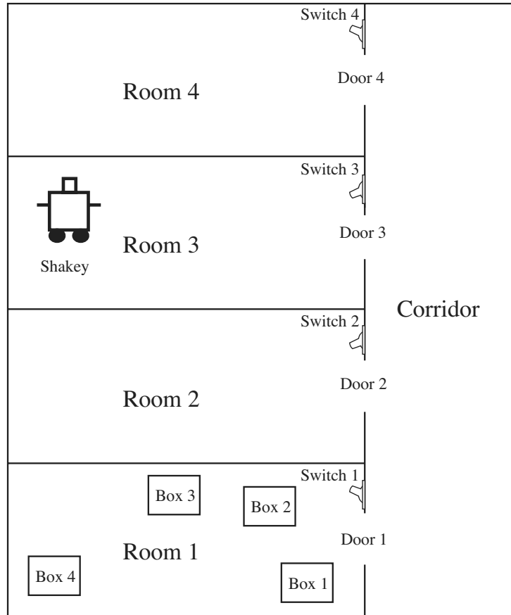
Figure 10.14 Shakey's world. Shakey can move between landmarks within a room, can pass through the door between rooms, can climb climbable objects and push pushable objects, and can flip light switches.
