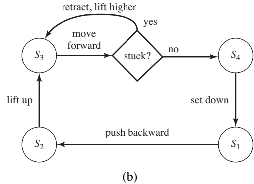
Figure 25.24 (a) Genghis, a hexapod robot. (b) An augmented finite state machine (AFSM) for the control of a single leg. Notice that this AFSM reacts to sensor feedback: if a leg is stuck during the forward swinging phase, it will be lifted increasingly higher.
