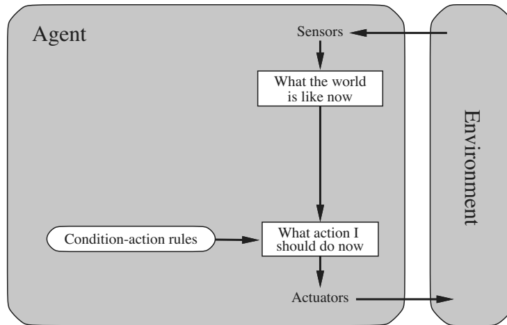
Figure 2.9 Schematic diagram of a simple reflex agent.
