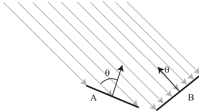
Figure 24.5 Two surface patches are illuminated by a distant point source, whose rays are shown as gray arrowheads. Patch A is tilted away from the source ( \theta is close to 90^\circ ) and collects less energy, because it cuts fewer light rays per unit surface area. Patch B, facing the source ( \theta is close to 0^\circ ), collects more energy.
