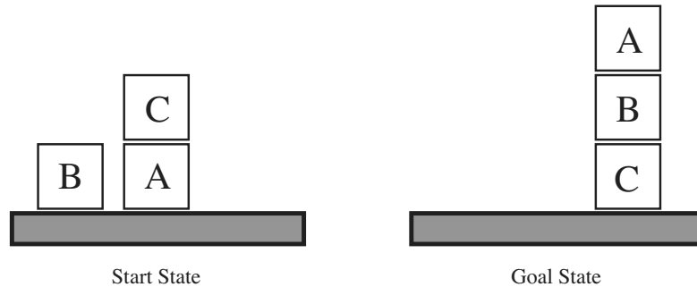
Figure 10.4 Diagram of the blocks-world problem in Figure 10.3.
