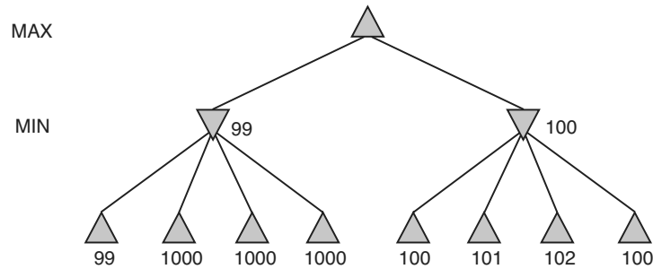
Figure 5.14 A two-ply game tree for which heuristic minimax may make an error.
