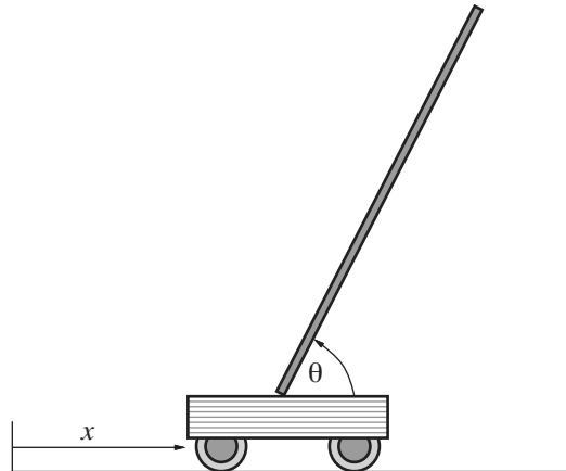
Figure 21.9 Setup for the problem of balancing a long pole on top of a moving cart. The cart can be jerked left or right by a controller that observes x , \theta , \dot{x} , and \dot{\theta} .
