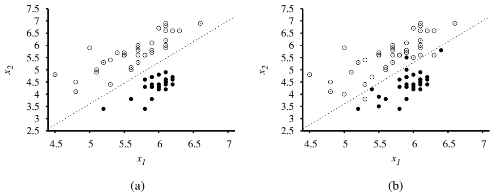
Figure 18.15 (a) Plot of two seismic data parameters, body wave magnitude x_1 and surface wave magnitude x_2 , for earthquakes (white circles) and nuclear explosions (black circles) occurring between 1982 and 1990 in Asia and the Middle East (Kebeasy et al. , 1998). Also shown is a decision boundary between the classes. (b) The same domain with more data points. The earthquakes and explosions are no longer linearly separable.
