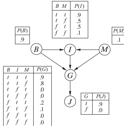
Figure 14.23 A simple Bayes net with Boolean variables B = BrokeElectionLaw , I = Indicted , M = PoliticallyMotivatedProsecutor , G = FoundGuilty , J = Jailed .
