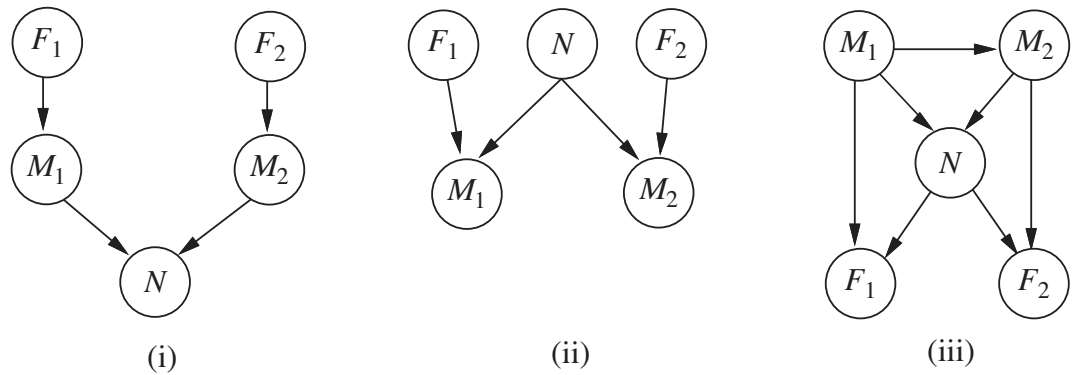
Figure 14.22 Three possible networks for the telescope problem.
