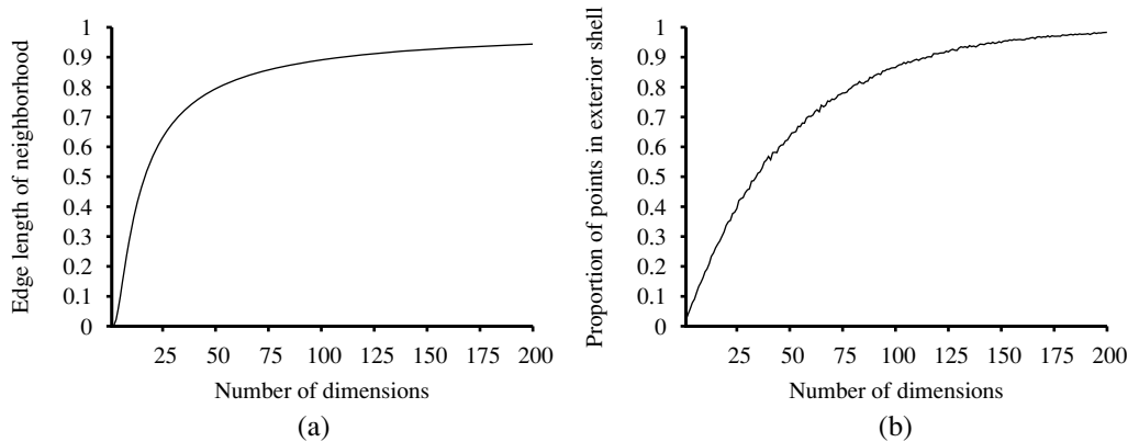
Figure 18.27 The curse of dimensionality: (a) The length of the average neighborhood for 10-nearest-neighbors in a unit hypercube with 1,000,000 points, as a function of the number of dimensions. (b) The proportion of points that fall within a thin shell consisting of the outer 1% of the hypercube, as a function of the number of dimensions. Sampled from 10,000 randomly distributed points.
