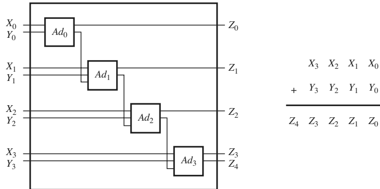
Figure 8.8 A four-bit adder. Each Ad_i is a one-bit adder, as in Figure 8.6 on page 309.
