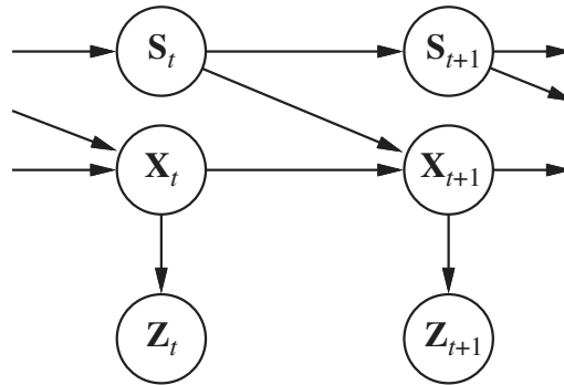
Figure 15.21 A Bayesian network representation of a switching Kalman filter. The switching variable S_t is a discrete state variable whose value determines the transition model for the continuous state variables \mathbf{X}_t . For any discrete state i , the transition model \mathbf{P}(\mathbf{X}_{t+1}|\mathbf{X}_t, S_t = i) is a linear Gaussian model, just as in a regular Kalman filter. The transition model for the discrete state, \mathbf{P}(S_{t+1}|S_t) , can be thought of as a matrix, as in a hidden Markov model.
