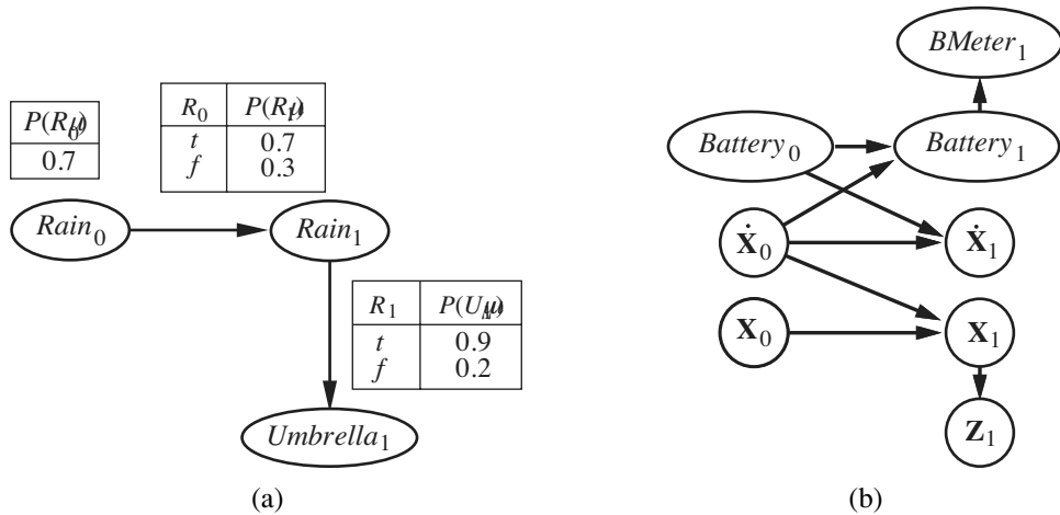
Figure 15.13 (a) Specification of the prior, transition model, and sensor model for the umbrella DBN. All subsequent slices are assumed to be copies of slice 1. (b) A simple DBN for robot motion in the X–Y plane.
