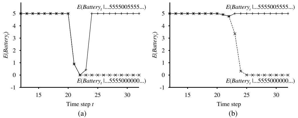
Figure 15.14 (a) Upper curve: trajectory of the expected value of Battery_t for an observation sequence consisting of all 5s except for 0s at t = 21 and t = 22 , using a simple Gaussian error model. Lower curve: trajectory when the observation remains at 0 from t = 21 onwards. (b) The same experiment run with the transient failure model. Notice that the transient failure is handled well, but the persistent failure results in excessive pessimism about the battery charge.
