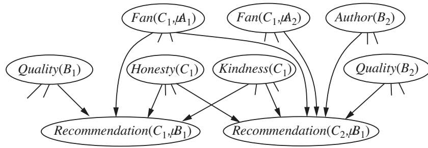
Figure 14.19 Fragment of the equivalent Bayes net when Author(B_2) is unknown.
