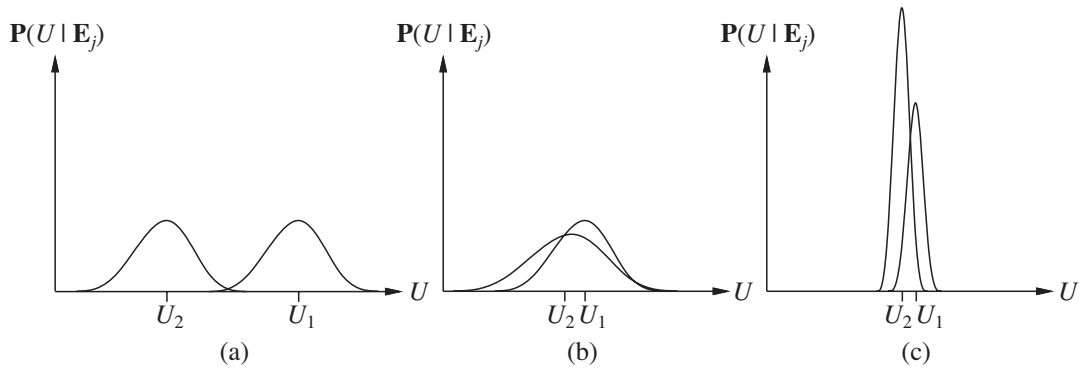
Figure 16.8 Three generic cases for the value of information. In (a), a_1 will almost certainly remain superior to a_2 , so the information is not needed. In (b), the choice is unclear and the information is crucial. In (c), the choice is unclear, but because it makes little difference, the information is less valuable. (Note: The fact that U_2 has a high peak in (c) means that its expected value is known with higher certainty than U_1 .)
