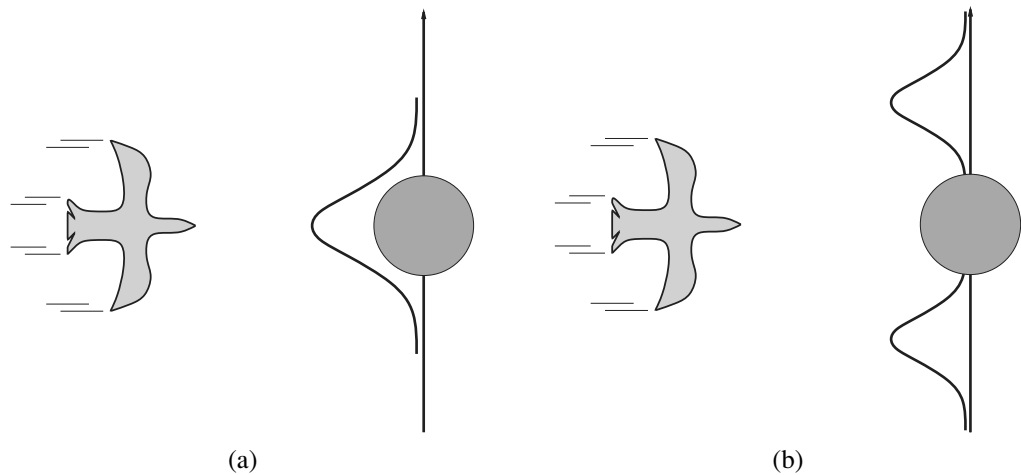
Figure 15.12 A bird flying toward a tree (top views). (a) A Kalman filter will predict the location of the bird using a single Gaussian centered on the obstacle. (b) A more realistic model allows for the bird's evasive action, predicting that it will fly to one side or the other.
