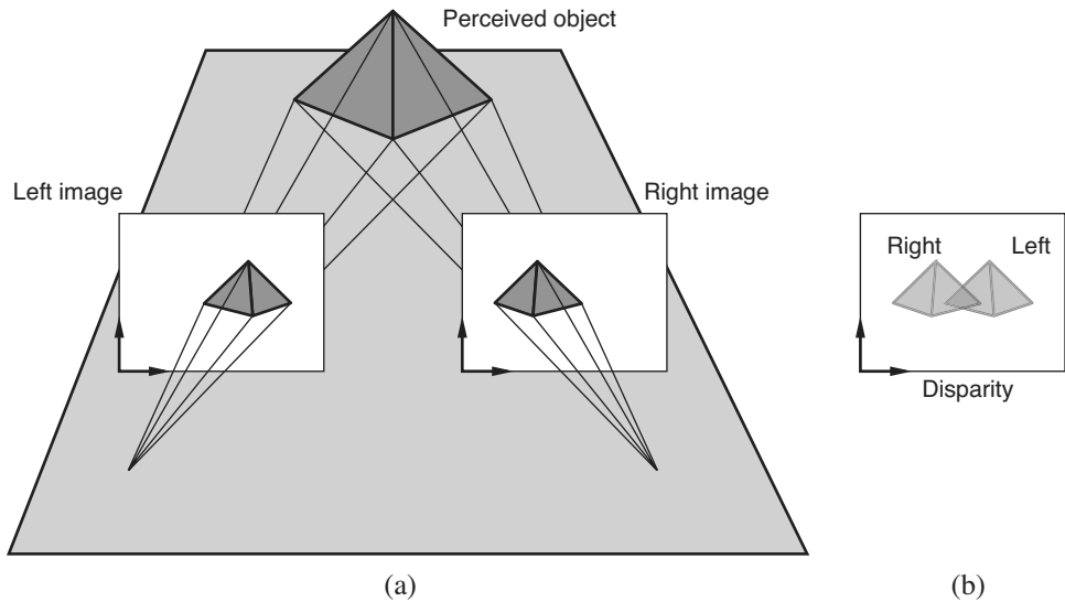
Figure 24.16 Translating a camera parallel to the image plane causes image features to move in the camera plane. The disparity in positions that results is a cue to depth. If we superimpose left and right image, as in (b), we see the disparity.
