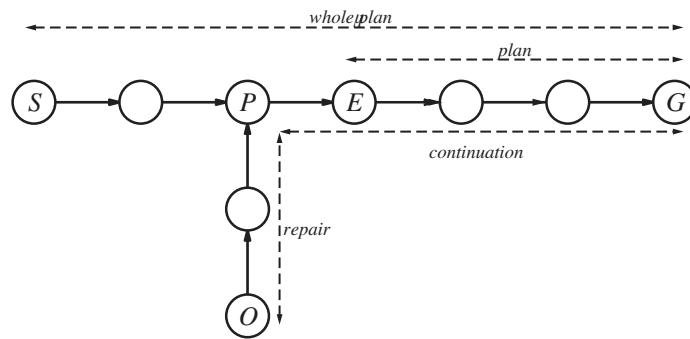
Figure 11.9 Before execution, the planner comes up with a plan, here called whole plan , to get from S to G . The agent executes steps of the plan until it expects to be in state E , but observes it is actually in O . The agent then replans for the minimal repair plus continuation to reach G .
