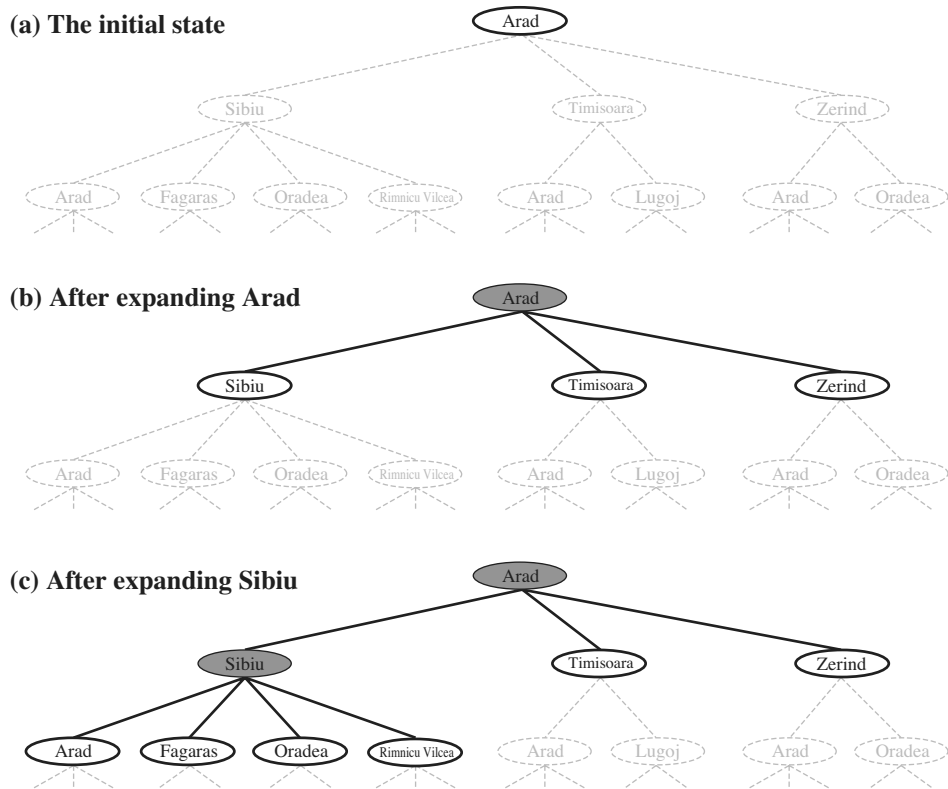
Figure 3.6 Partial search trees for finding a route from Arad to Bucharest. Nodes that have been expanded are shaded; nodes that have been generated but not yet expanded are outlined in bold; nodes that have not yet been generated are shown in faint dashed lines.
