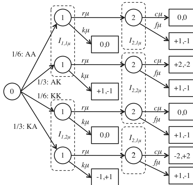
Figure 17.13 Extensive form of a simplified version of poker.
