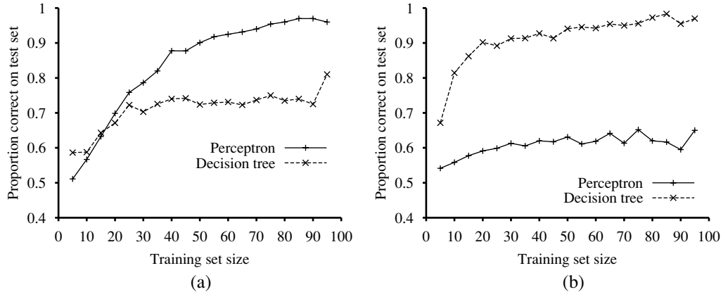
Figure 18.22 Comparing the performance of perceptrons and decision trees. (a) Perceptrons are better at learning the majority function of 11 inputs. (b) Decision trees are better at learning the WillWait predicate in the restaurant example.
