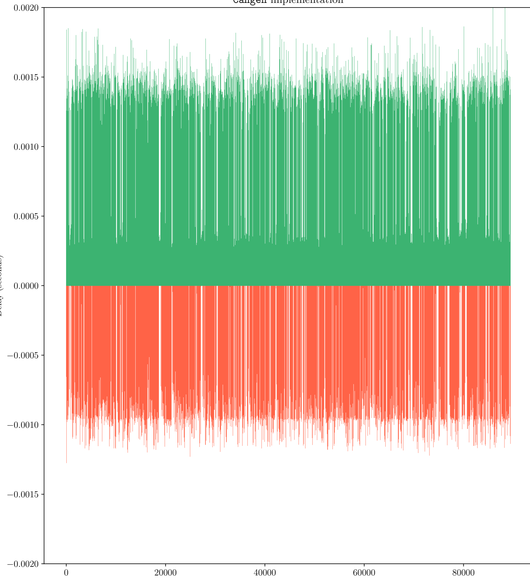
Cangen implementation
