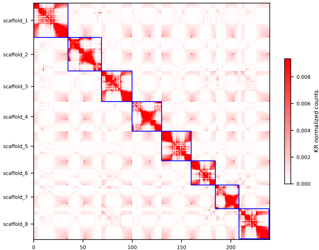
Hi-C contact map (bin size: 500 Kb, x-axis unit: Mb)
