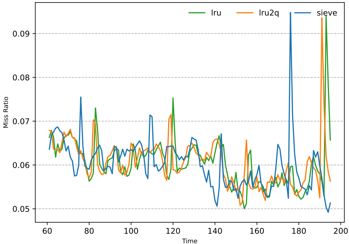
miss ratio after 60 mins-40GB_t20_lru,lru2q,sieve_195
