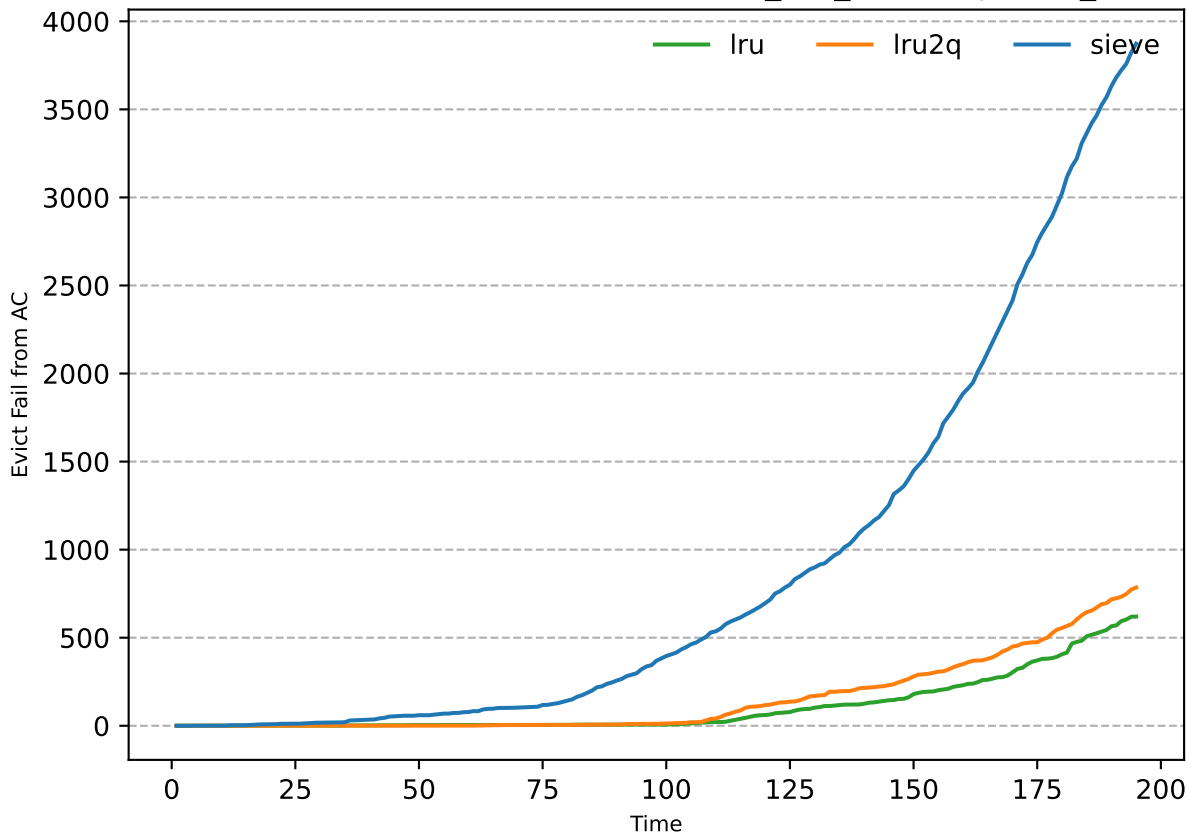
Evict Fail from Access Container-40GB_t20_lru,lru2q,sieve_195
