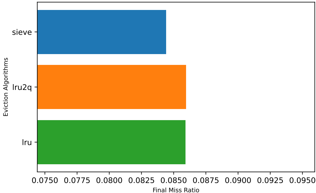
Final Miss Ratio-40GB_t20_lru,lru2q,sieve_195
