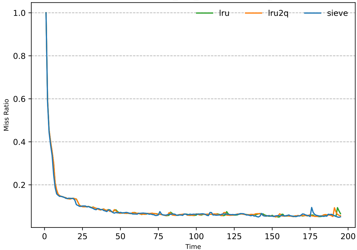
miss ratio-40GB_t20_lru,lru2q,sieve_195
