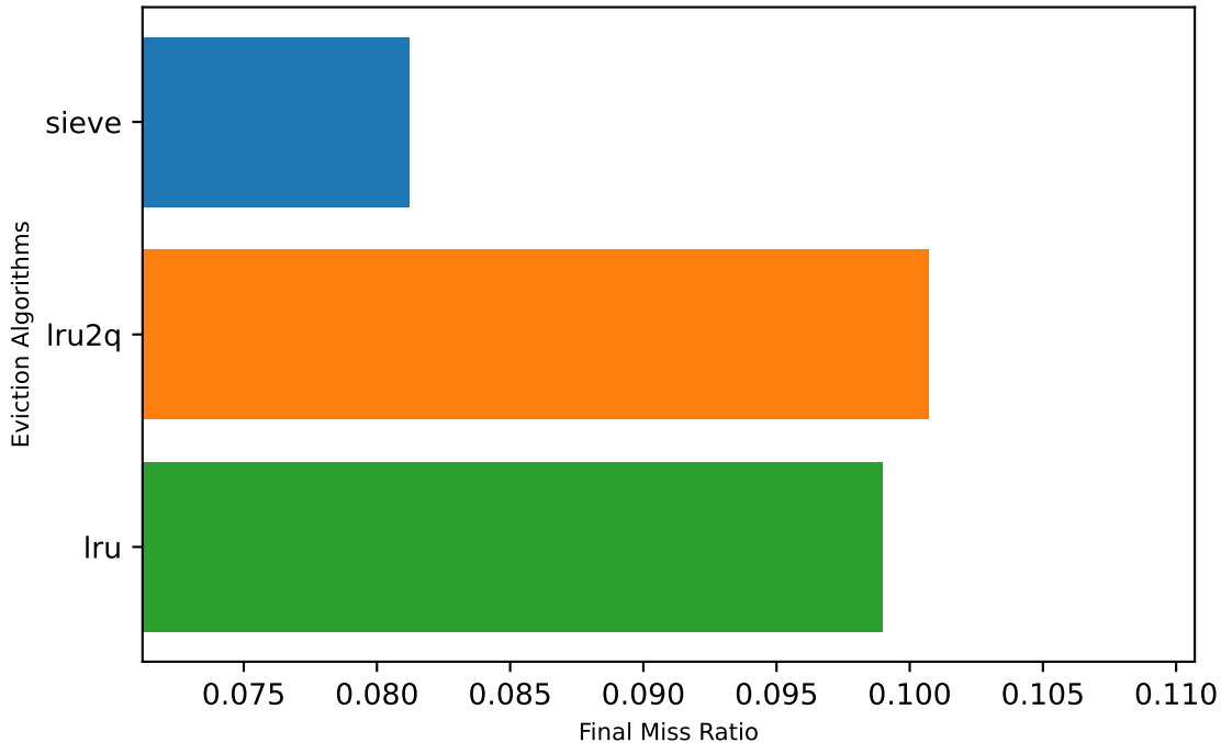
Final Miss Ratio-8192MB_t48_lru,lru2q,sieve
