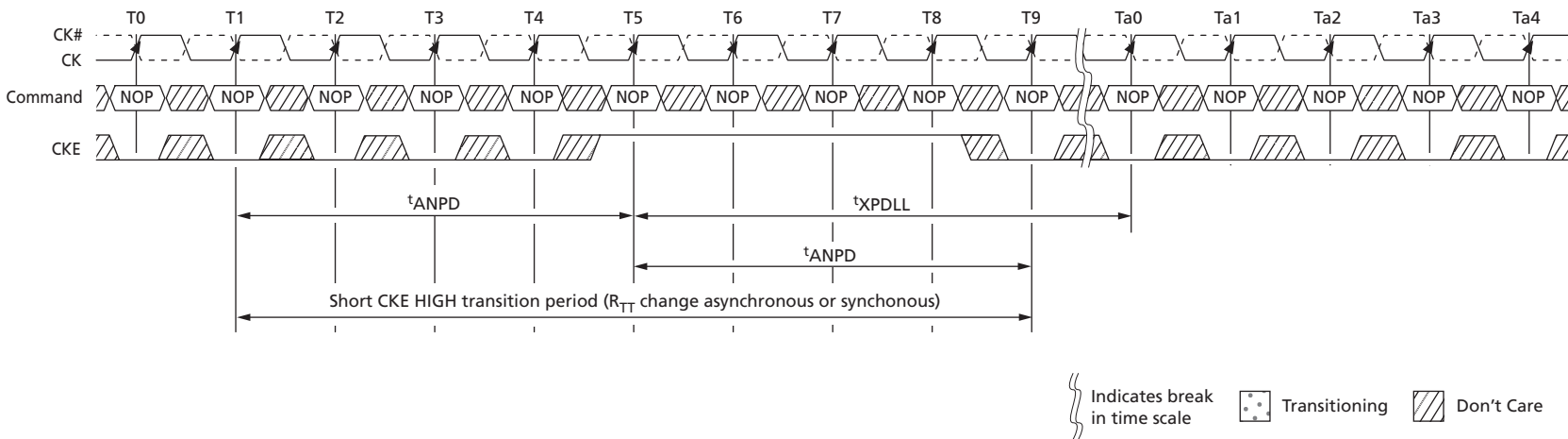
Figure 115: Transition Period for Short CKE HIGH Cycles with Entry and Exit Period Overlapping
