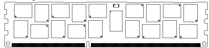
Figure 1: 240-Pin RDIMM (R/C E2)
