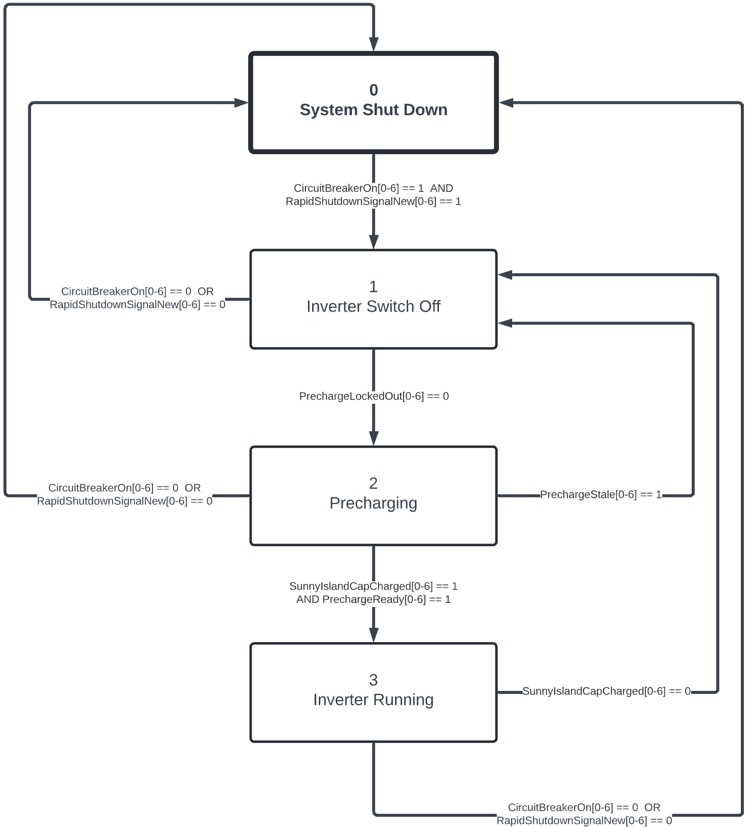
Battery Protection Control Circuit Arduino Code: State Machine Diagram
