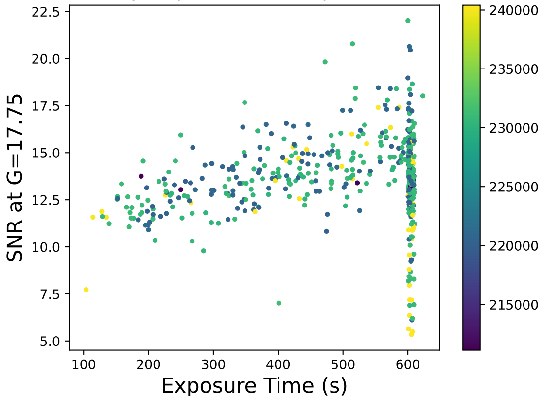
Single Exposures, Colored by ObsDate
