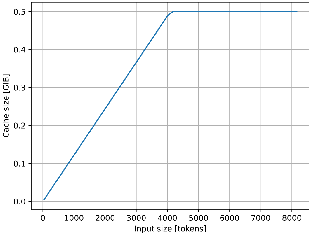
DynamicSlidingWindowCache
