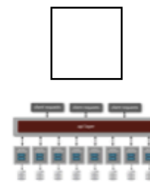
microservices
