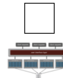
service-based
