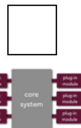
microkernel
