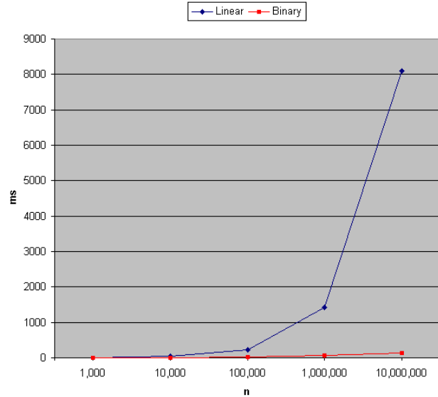
Figure 8: Performance of Linear vs. Binary search algorithms.
