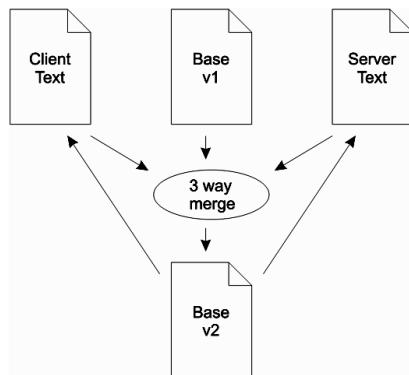
Figure 1: Three-way merge.
