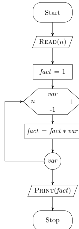
Figure 2.7: To find the factorial of a number
