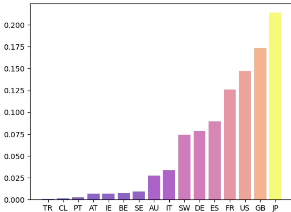
Figure 121. Eigenvector centrality
