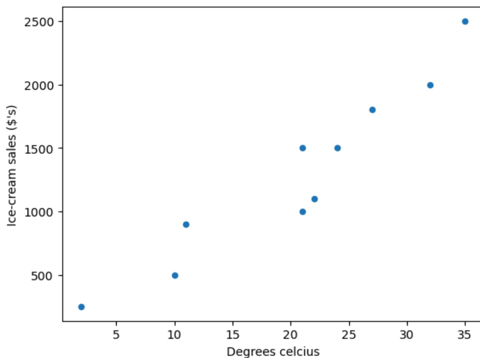
Figure 123. Scatter plot
