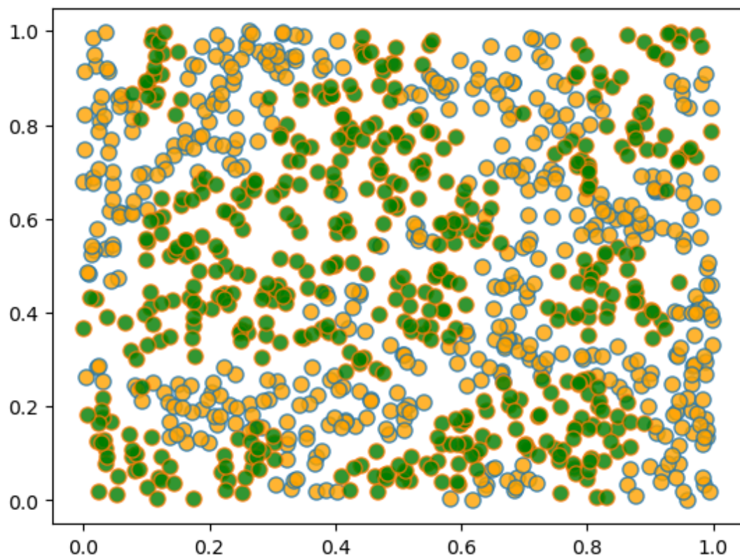
iteration 20000
