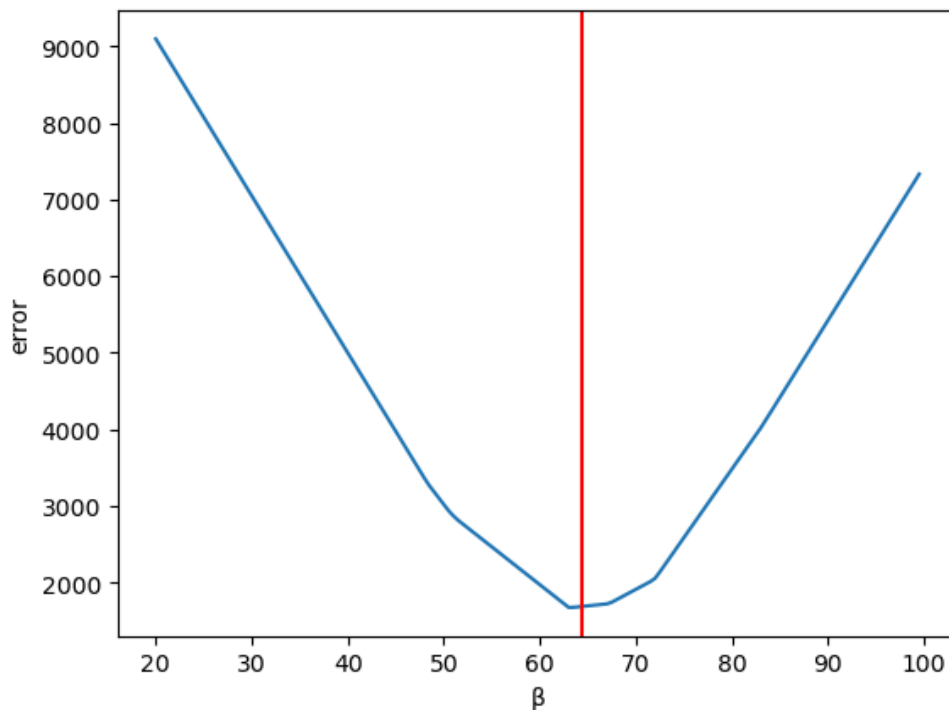
Figure 128. Plotting the error
