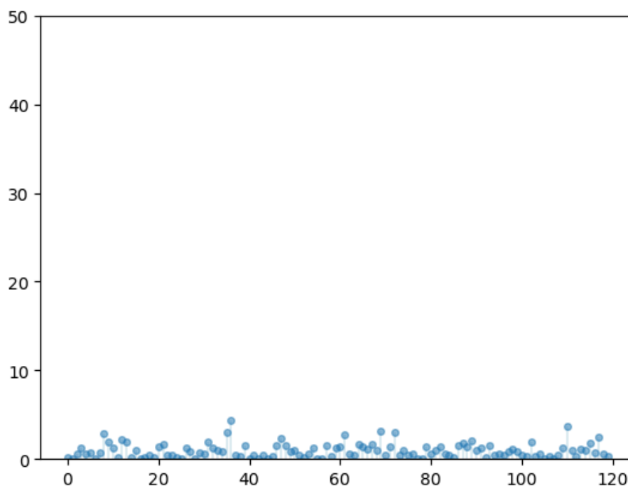
Figure 91. Draws of exponential distribution
