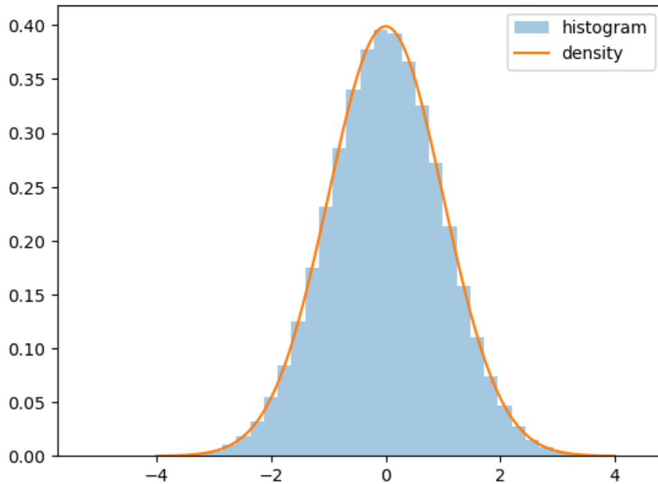
Figure 85. Histogram of observations
