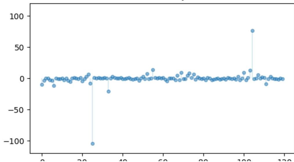
draws from the Cauchy distribution
