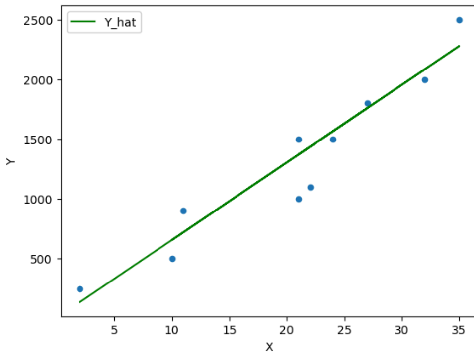
Figure 126. Scatter plot with a line of fit #3
