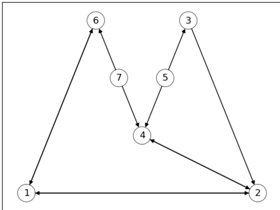
Figure 120. Sample Graph
