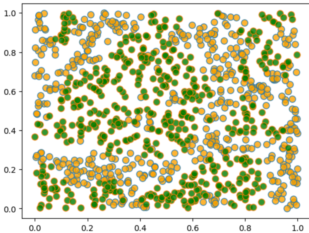
iteration 40000
