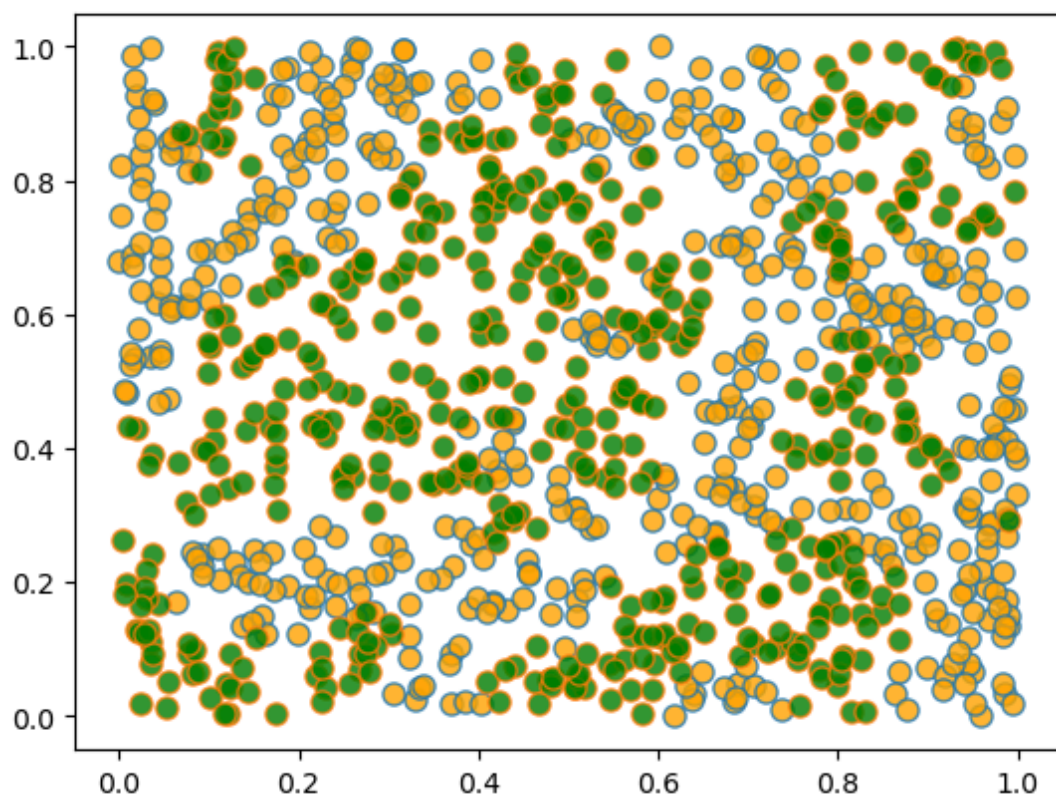
iteration 10000
