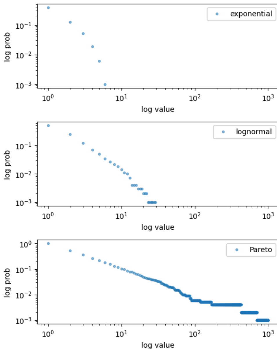
Figure 95. Empirical CCDFs
