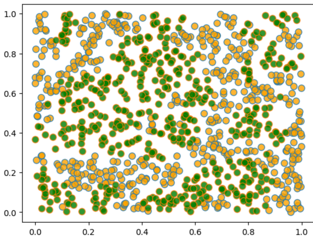
iteration 30000
