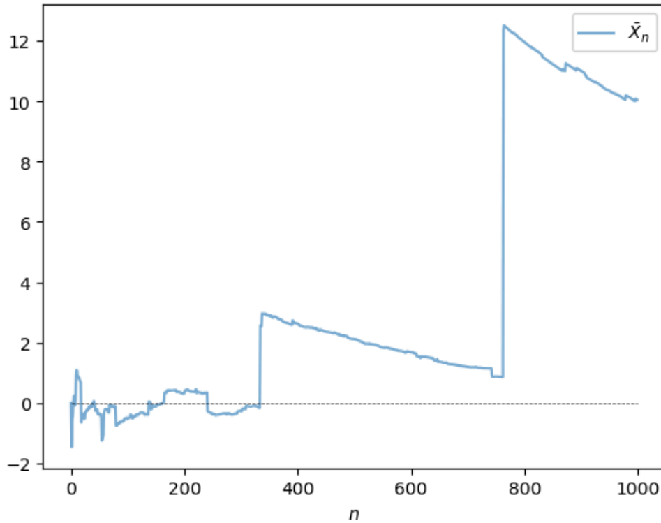
Figure 100. LLN failure
