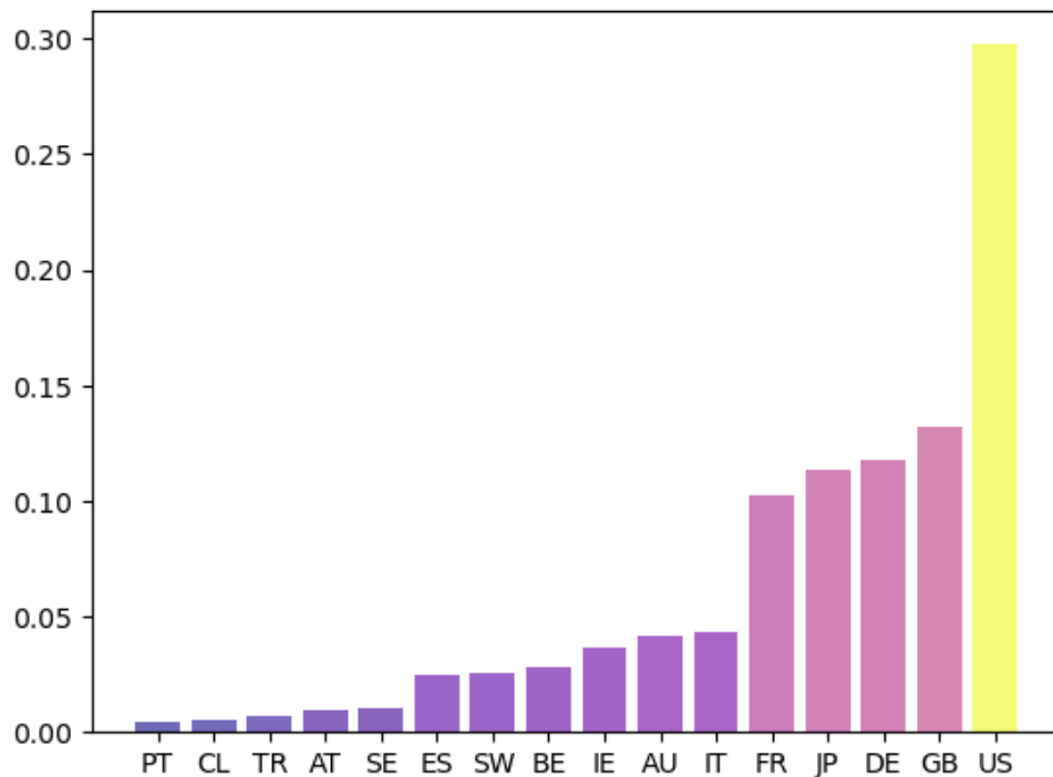
Figure 122. Eigenvector authority
