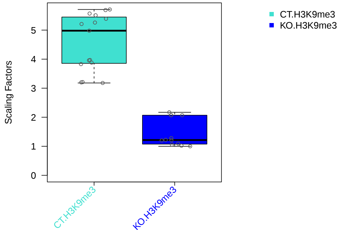
ScalingFactor ~ All antibodies
