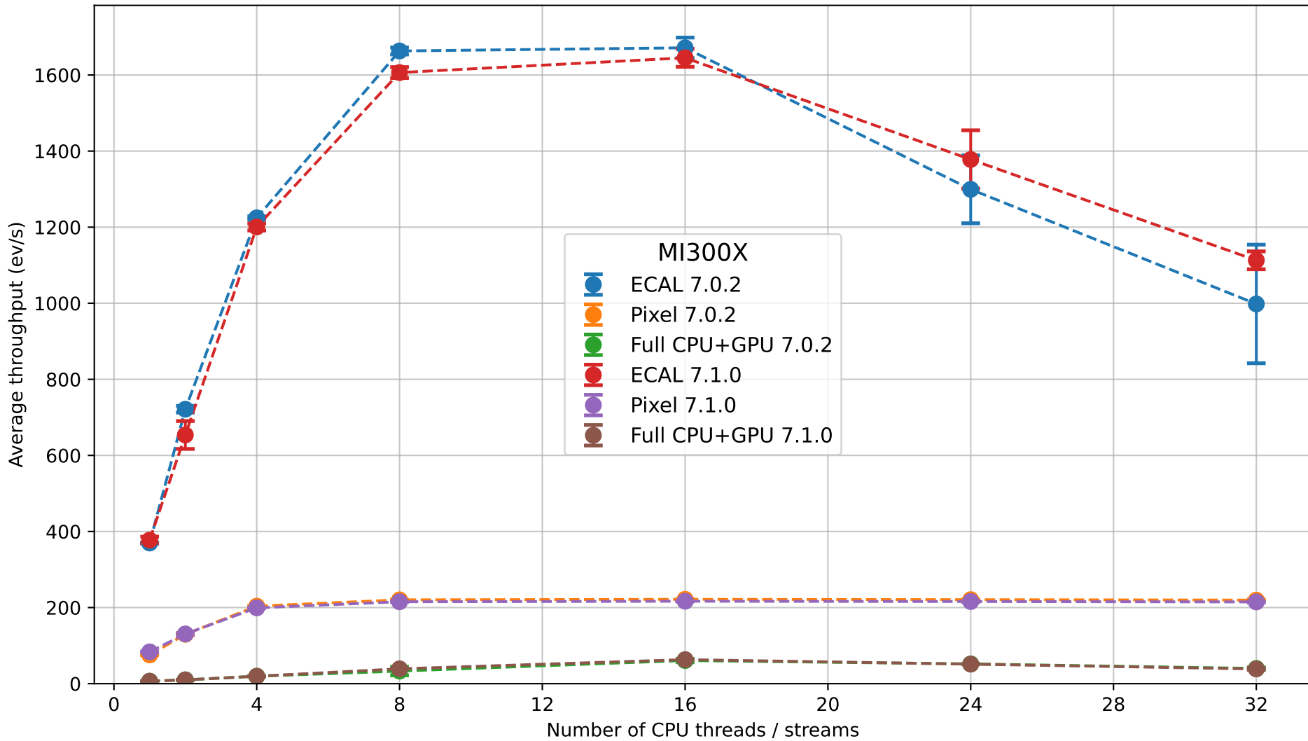
Average throughput vs number of CPU threads per job
